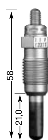
Y-207 T M 12 x 1.25 12 Hex 11 V
