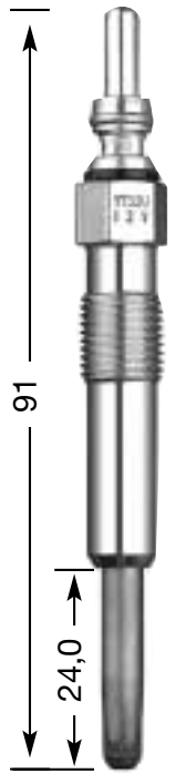
Y-732 U M 10 x 1 10 Hex 12 V
