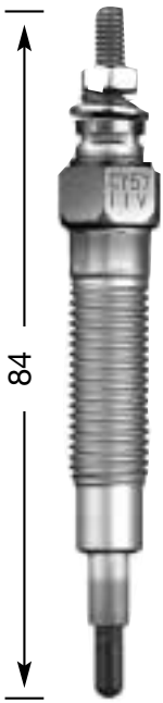
CY 57 M 10 x 1.25 12 Hex 11 V
