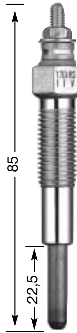
Y-701 RS M 10 x 1,25 12 Hex 11 V
