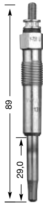
Y-731 U M 10 x 1 10 Hex 11 V
