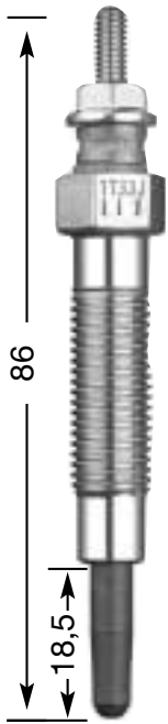
Y-733 J M 10 x 1.25 12 Hex 11 V
