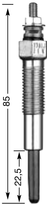
Y-701 J M 10 x 1,25 12 Hex 11 V
