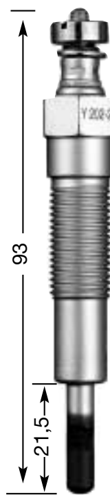
Y-202-2 M 12 x 1.25 14 Hex
