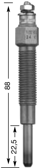
Y-757 RS M 10 x 1.25 12 Hex 24 V
