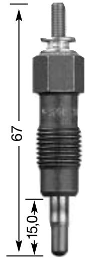
Y-926 U M 12 x 1.25 12 Hex 11 V
