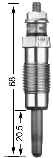
Y-935 U M 12 x 1.25 12 Hex 11 V
