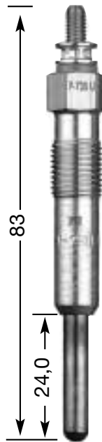
Y-730 U M 10 x 1 10 Hex 11 V
