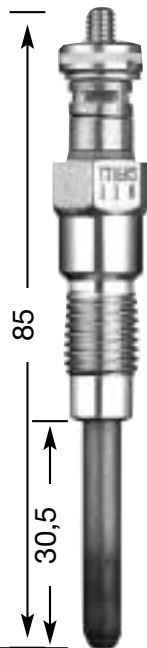
Y-716 RS M 10 x 1.25 12 Hex 11 V
