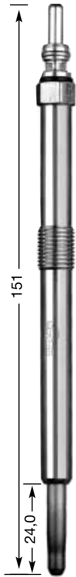
Y-517 J M 10 x 1 10 Hex 11 V
