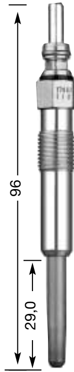
Y-741 U M 10 x 1 10 Hex 11 V
