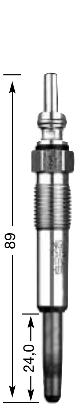
Y-515 J M 10 x 1 10 Hex 11 V
