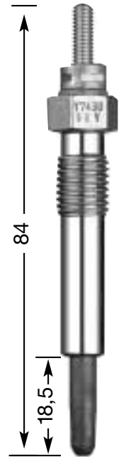
Y-743 U M 10 x 1.25 12 Hex 11 V
