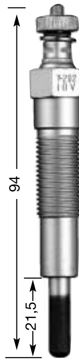
Y-202 M 12 x 1.25 14 Hex 10 V
