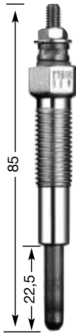
Y-701 R M 10 x 1,25 12 Hex 11 V
