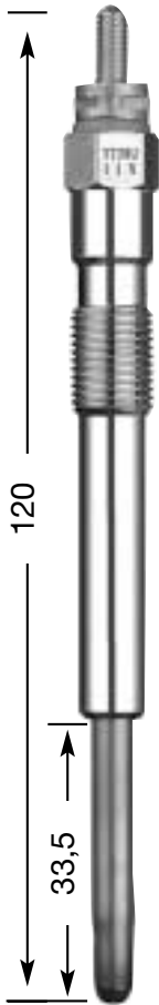
Y-738 U M 10 x 1 10 Hex 11 V
