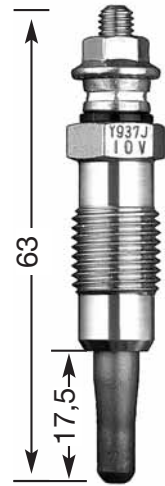
Y-937 J M 12 x 1.25 12 Hex 10 V
