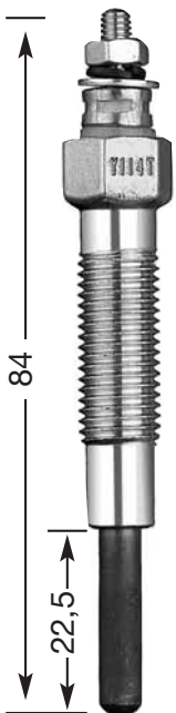
Y-114 T M 10 x 1.25 12 Hex
