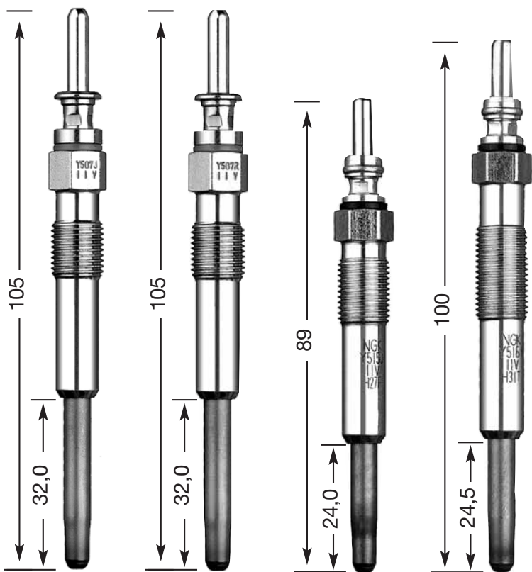
Y-507 J M 10 x 1 10 Hex 11 V
