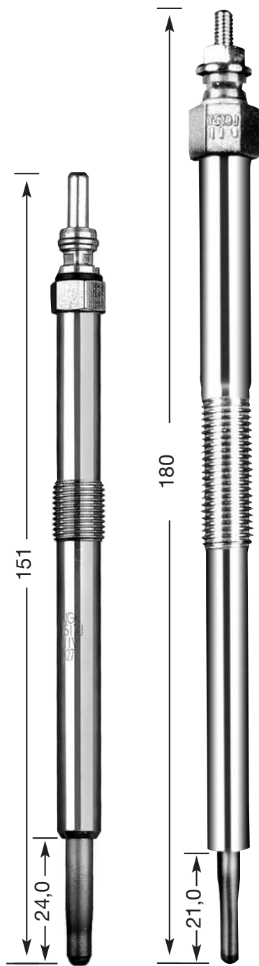
Y-517 J M 10 x 1 10 Hex 11 V
