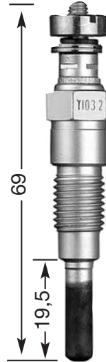
Y-103-2A M 10 x 1.25 12 Hex
