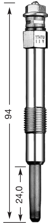
Y-747 U M 10 x 1 10 Hex 11 V
