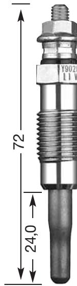
Y-902 R M 12 x 1.25 12 Hex 11 V
