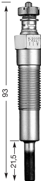
Y-222 T M 12 x 1.25 14 Hex 11 V
