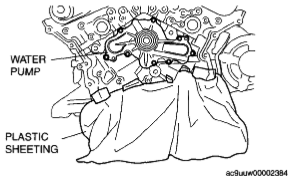
Fig. 21: View Of Water Pump And Plastic Sheetting Courtesy of MAZDA MOTORS CORP.
