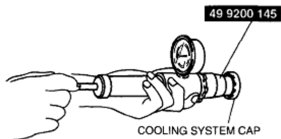
Fig. 10: Attaching Cooling System Cap To SST Courtesy of MAZDA MOTORS CORP.
