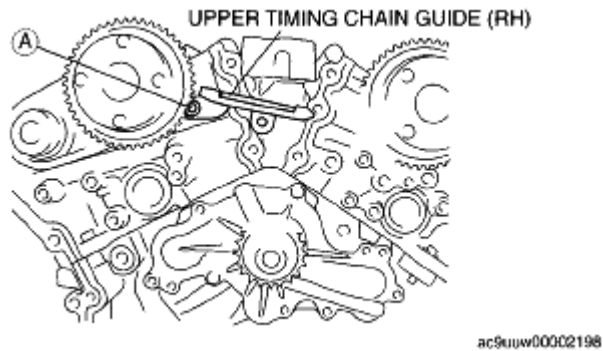
Fig. 20: Identifying Upper Timing Chain Guide Bolt Courtesy of MAZDA MOTORS CORP.
