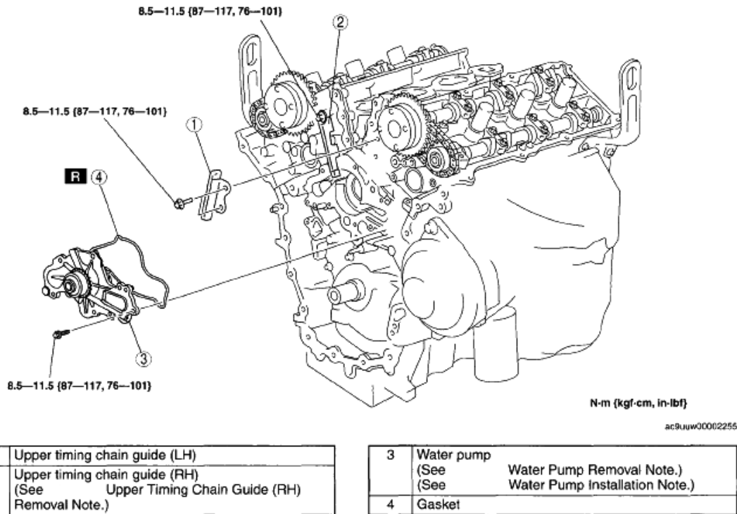
Fig. 18: Identifying Water Pump Components With Torque Specifications Courtesy of MAZDA MOTORS CORP.
