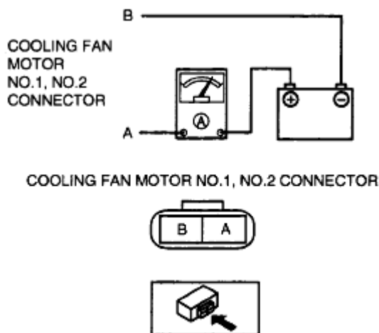
Fig. 24: Installing Tester And Battery To Cooling Fan Motor Connector (2 Terminals) Courtesy of MAZDA MOTORS CORP.
