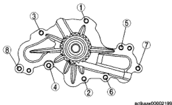
Fig. 22: Identifying Water Pump Bolts Tightening Sequence Courtesy of MAZDA MOTORS CORP.
