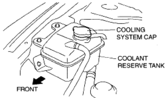
Fig. 7: Identifying Cooling System Cap Courtesy of MAZDA MOTORS CORP.
