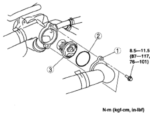
Fig. 15: Identifying Thermostat Cover And Thermostat With Torque Specifications Courtesy of MAZDA MOTORS CORP.
