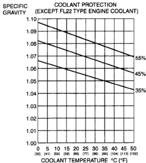
Fig. 5: Engine Coolant Protection Level Graph Courtesy of MAZDA MOTORS CORP.
