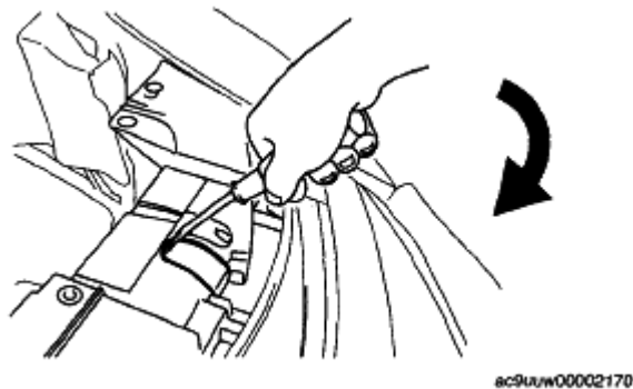
Fig. 14: Applying Downward Force Courtesy of MAZDA MOTORS CORP.
