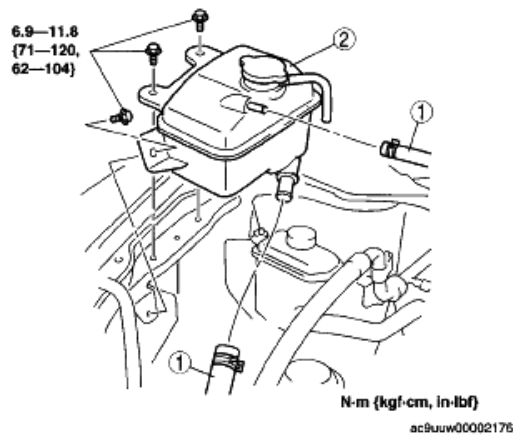
Fig. 11: Identifying Coolant Reserve Tank And Hose With Torque Specifications Courtesy of MAZDA MOTORS CORP.
