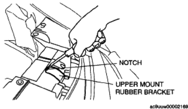
Fig. 13: Inserting Flathead Screwdriver Into Upper Mount Rubber Bracket Notch Courtesy of MAZDA MOTORS CORP.
