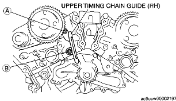
Fig. 19: Identifying Upper Timing Chain Guide Bolts Courtesy of MAZDA MOTORS CORP.
