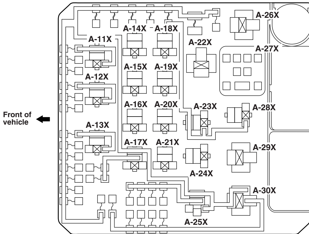
Relay box in engine room
