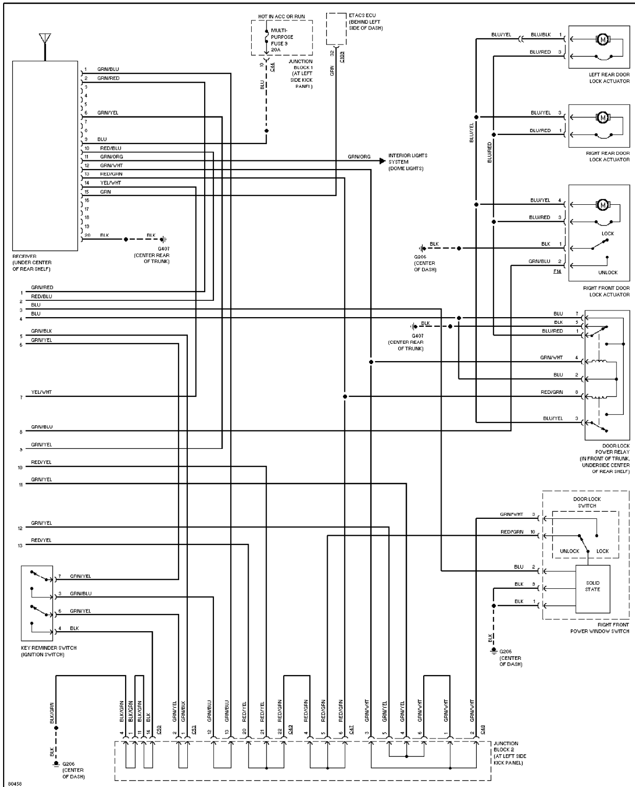
Power Door Lock Circuit, W/ Keyless Entry (2 of 2)
