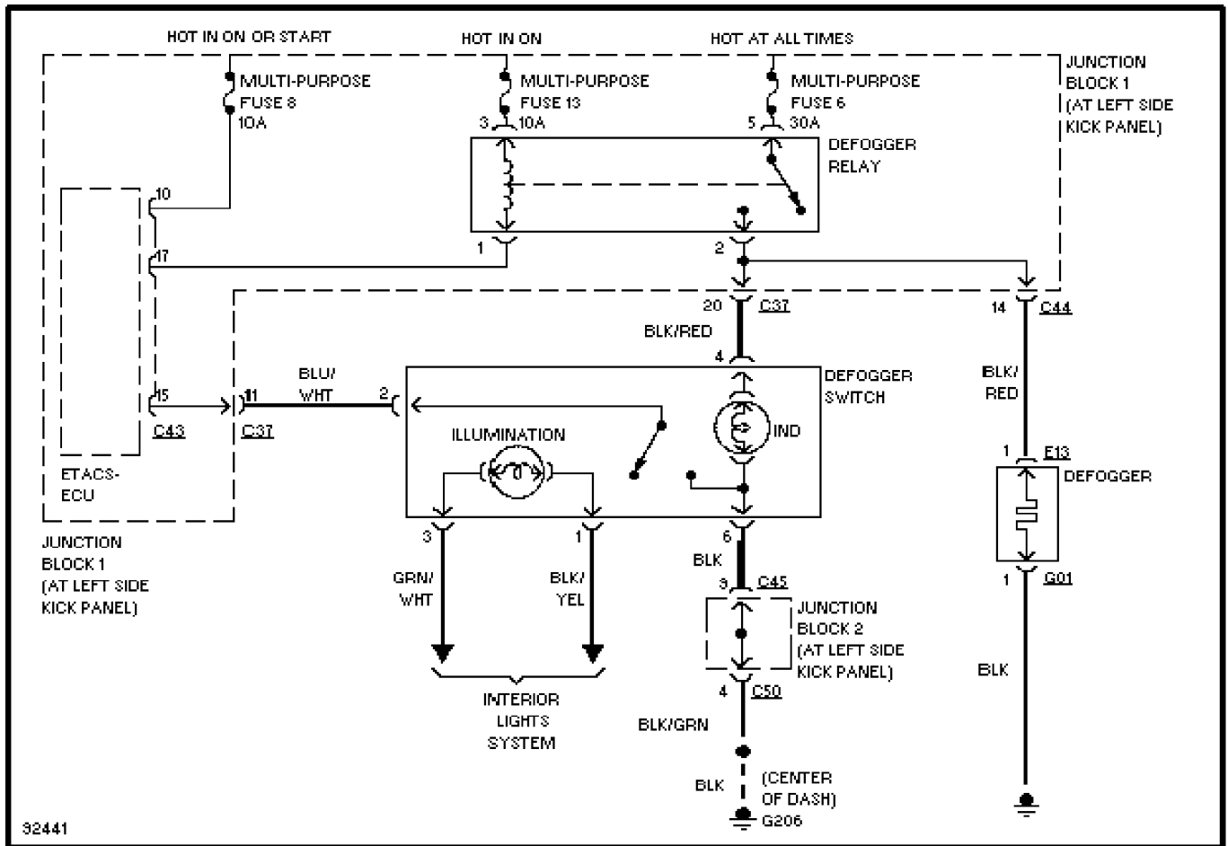
Defogger Circuit, W/ ETACS-ECU
