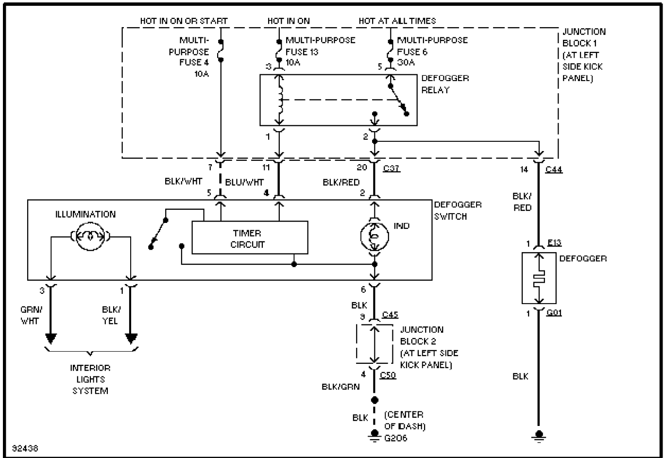
Defogger Circuit, W/O ETACS-ECU
