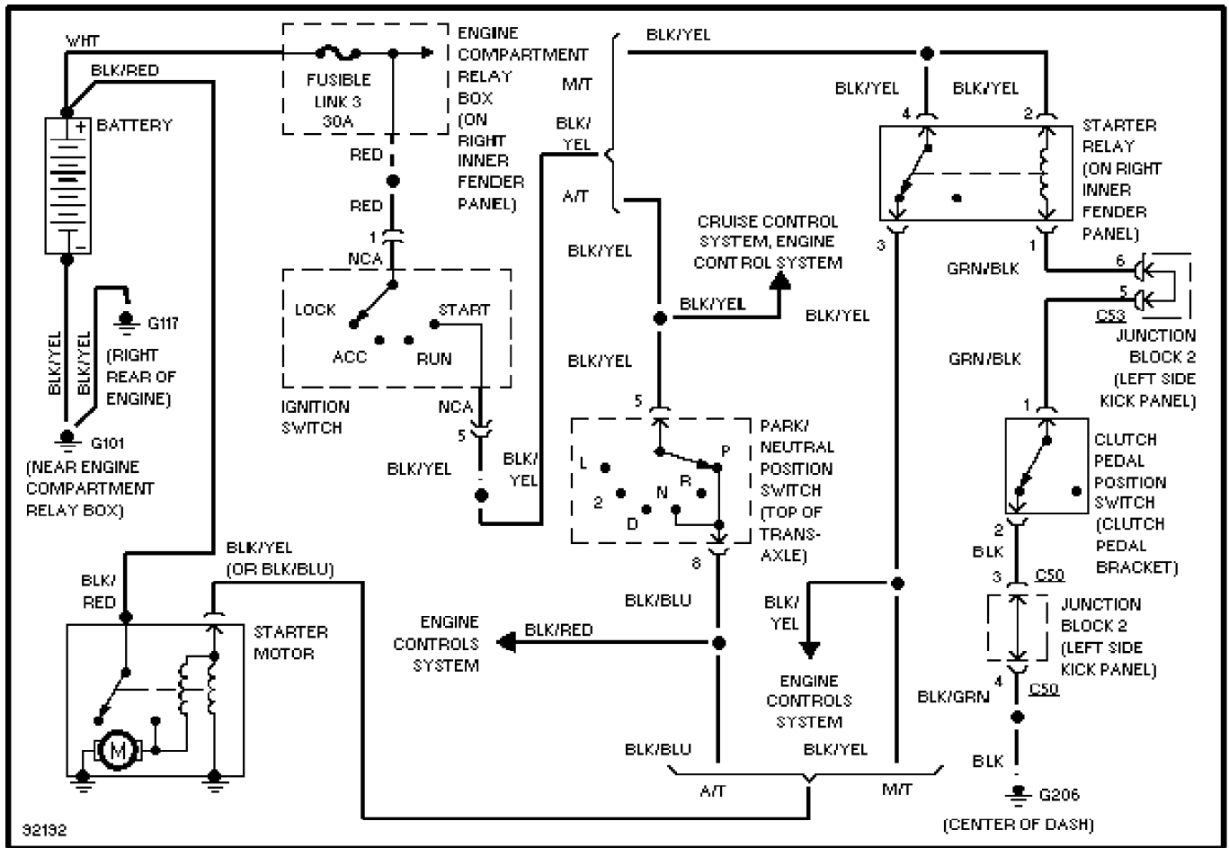
Starting Circuit, W/O Anti-theft
