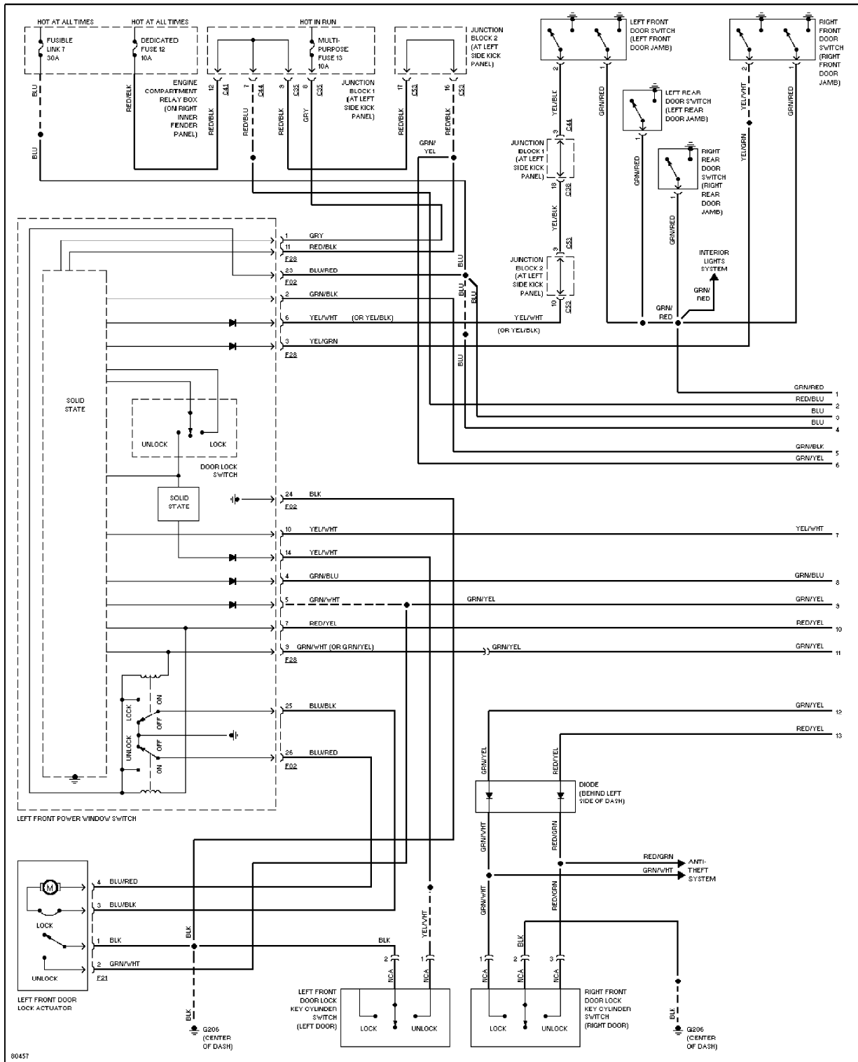
Power Door Lock Circuit, W/ Keyless Entry (1 of 2)
