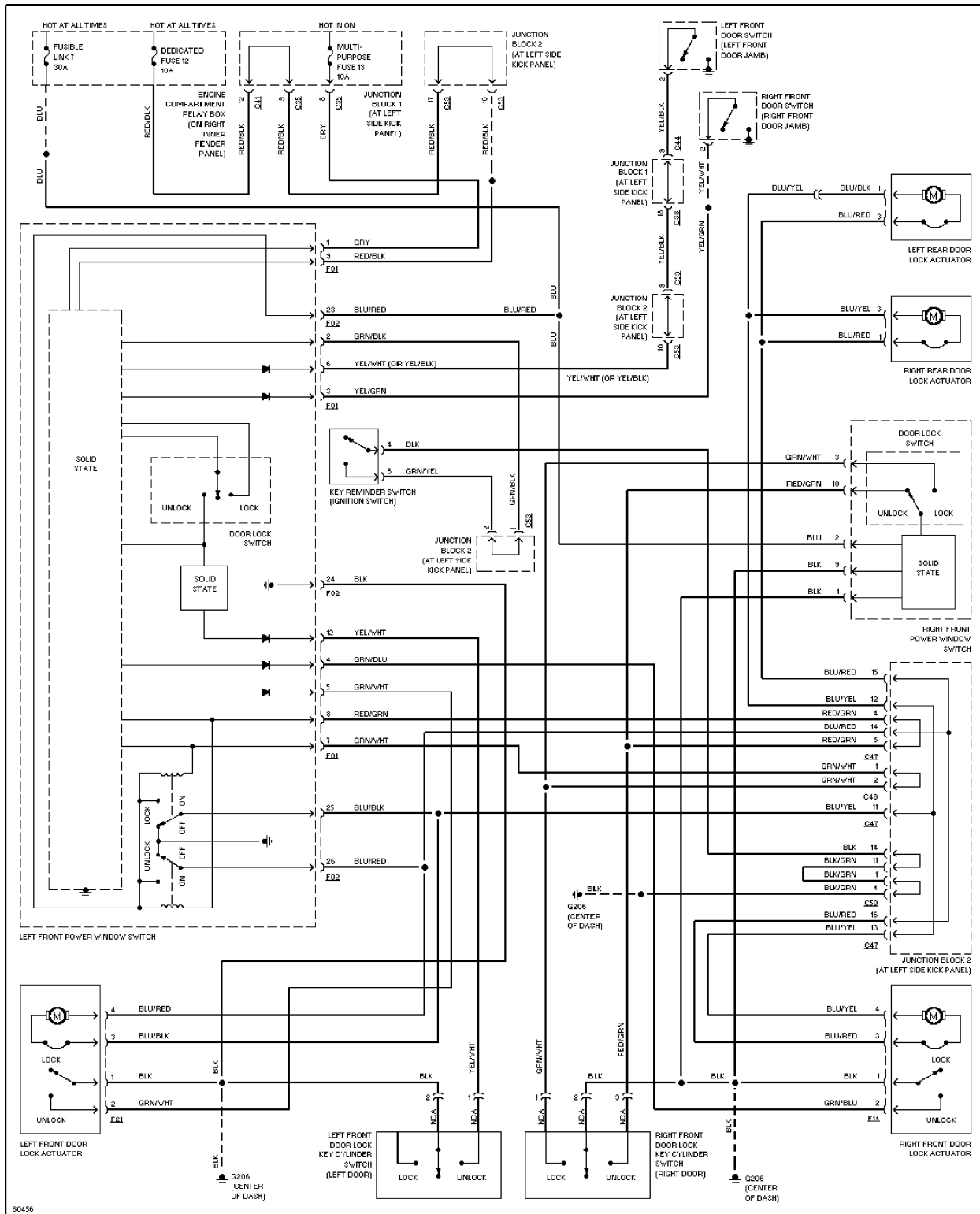
Power Door Lock Circuit, W/O Keyless Entry
