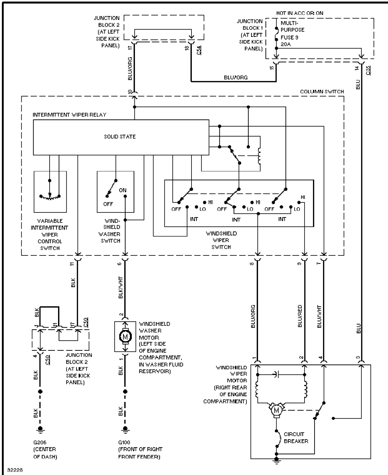
Wiper/Washer Circuit
