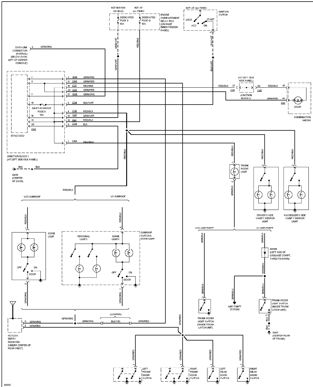
Courtesy Lamps Circuit, W/ ETACS-ECU
