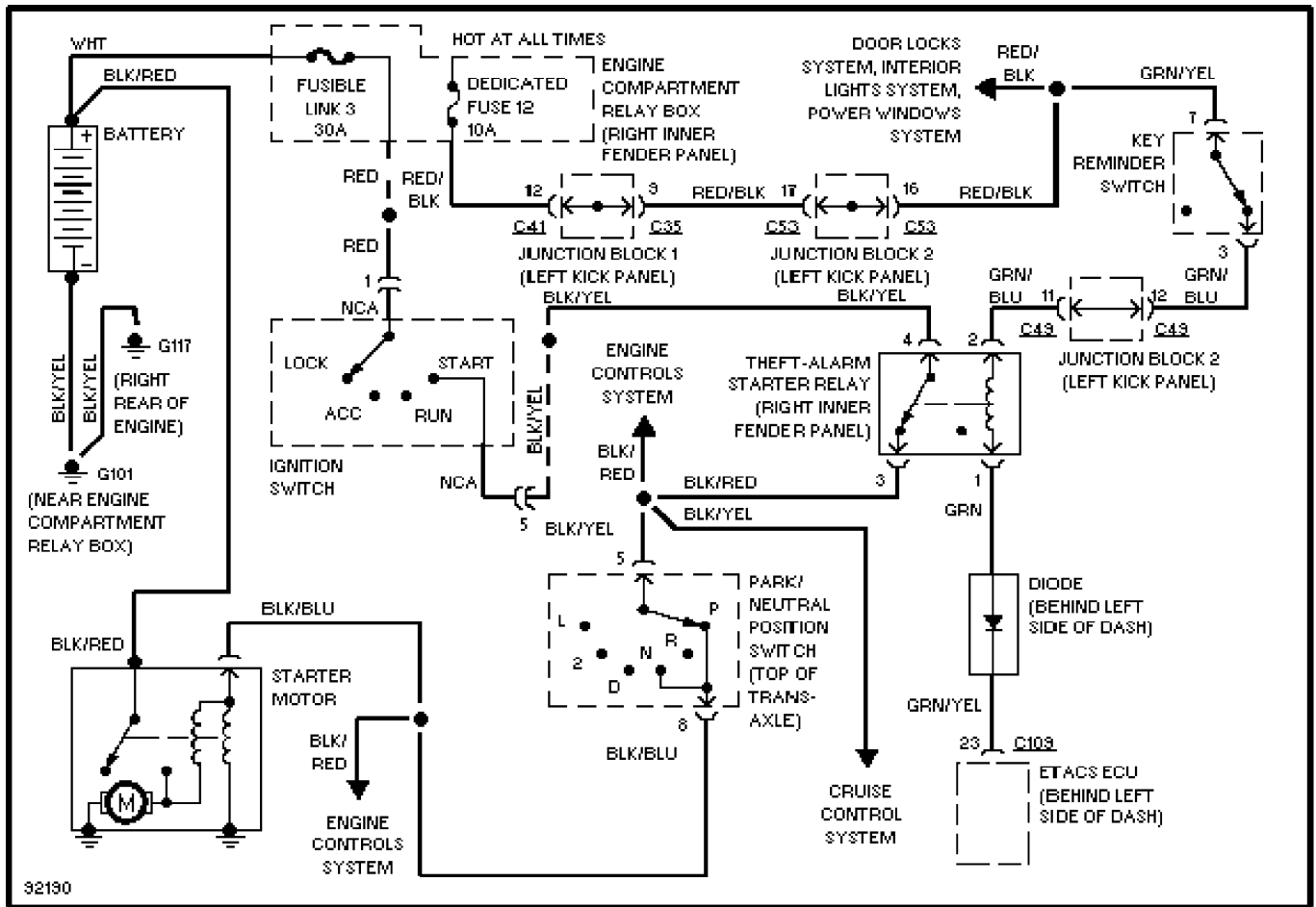
Starting Circuit, W/ Anti-theft
