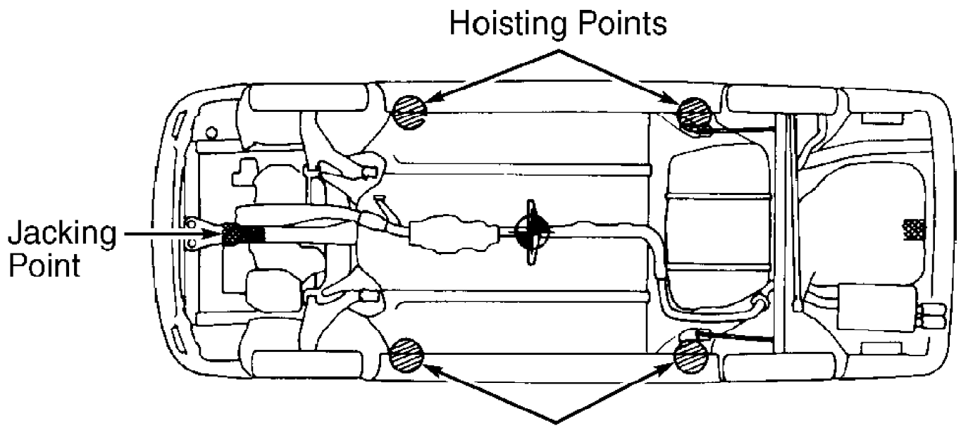
Hoisting Points 2WD
