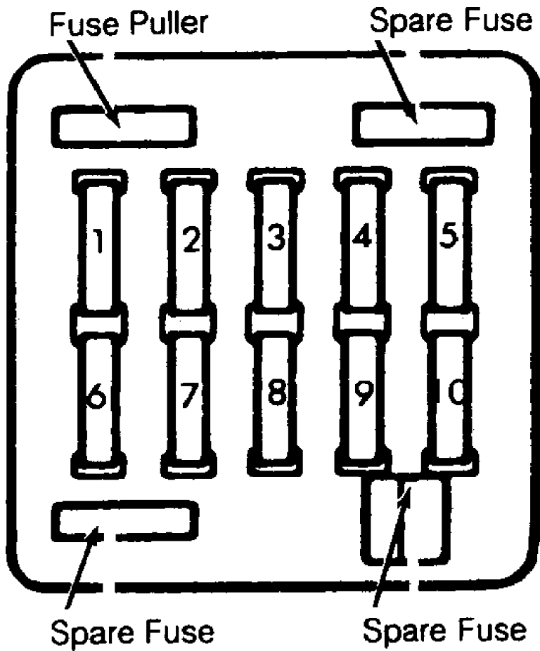
Fig. 1: Fuse Panel Identification (1983-91) Courtesy of Mitsubishi Motor Sales of America, Inc.
