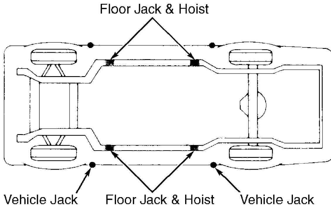
Fig. 1: Jacking & Hoisting Points (Typical)
