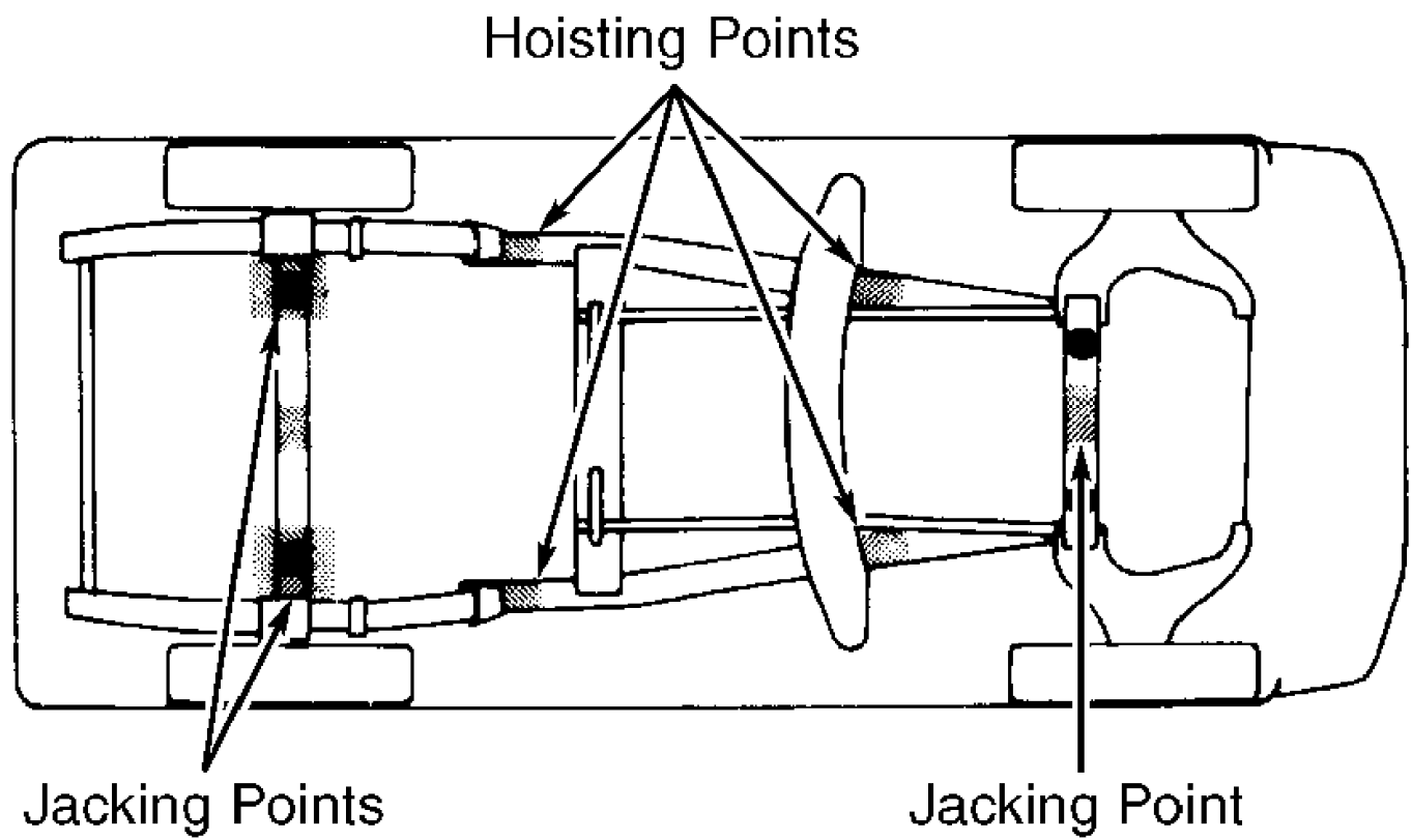
Fig. 2: Jacking & Hoisting Points (Montero) Courtesy of Mitsubishi Motor Sales of America.
