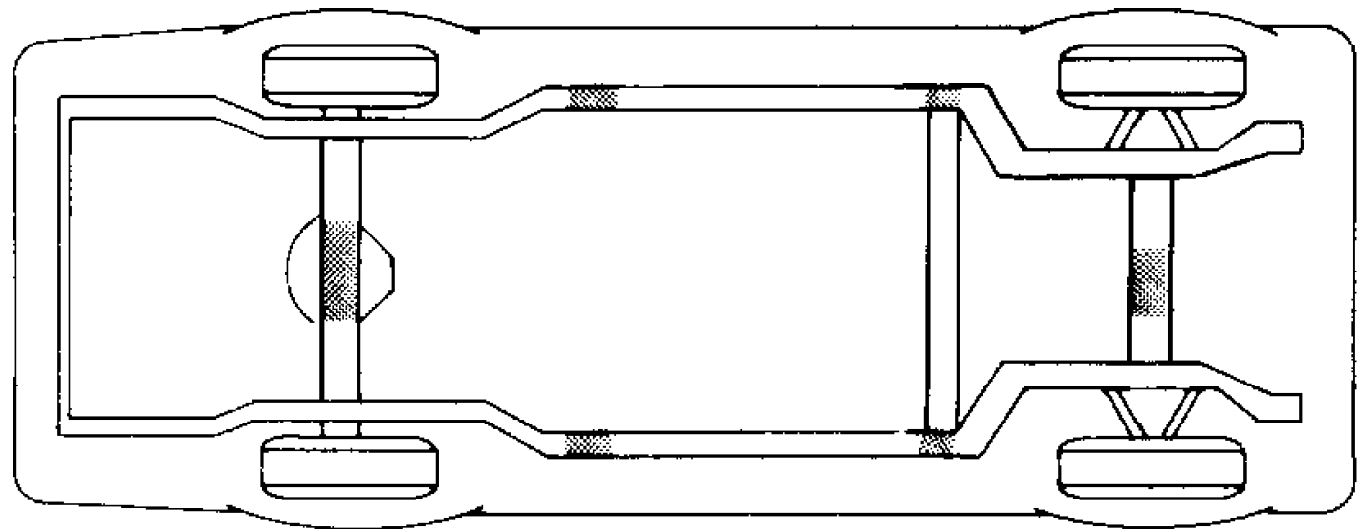
Fig. 2: Jacking & Hoisting Points (Montero) Courtesy of Mitsubishi Motor Sales of America.
