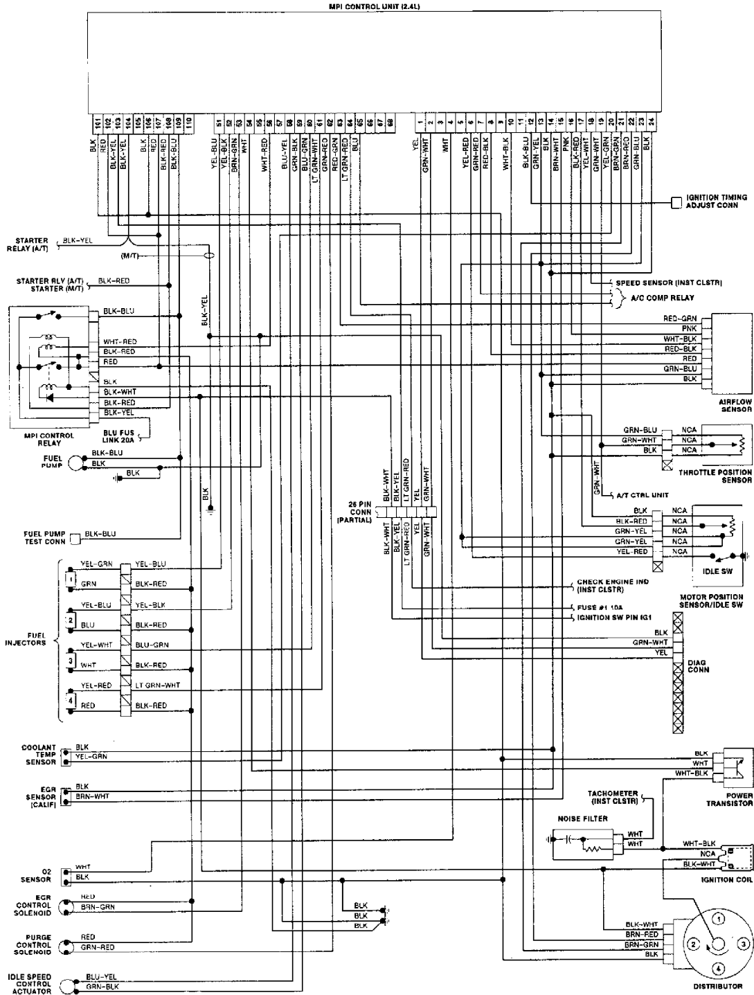
Fig. 11: Wiring Diagram (Pickup & Ram-50 2.4L)
