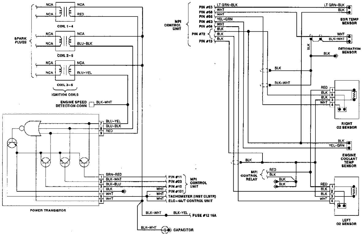
Fig. 17: Wiring Diagram (Stealth & 3000GT 3.0L - Turbo - 2 of 2)
