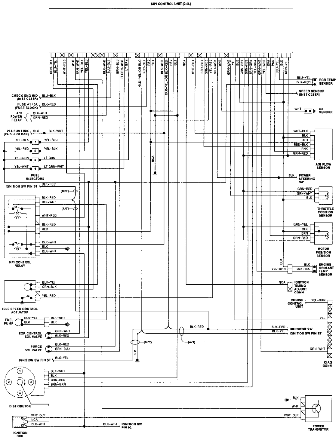
Fig. 2: Wiring Diagram (Colt Vista 2.0L)
