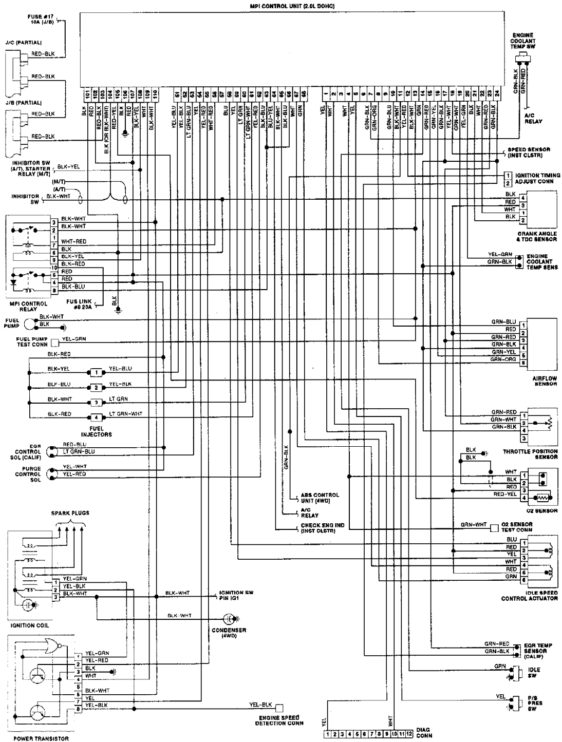
Fig. 7: Wiring Diagram (Galant 2.0L - DOHC)
