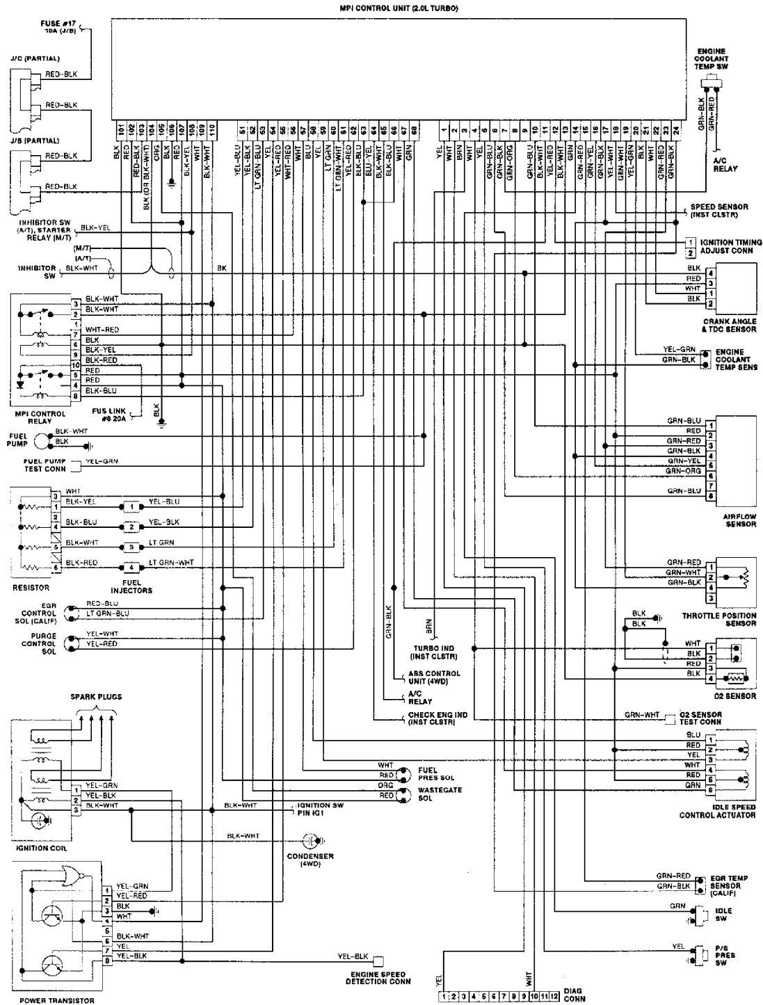
Fig. 8: Wiring Diagram (Galant 2.0L Turbo)
