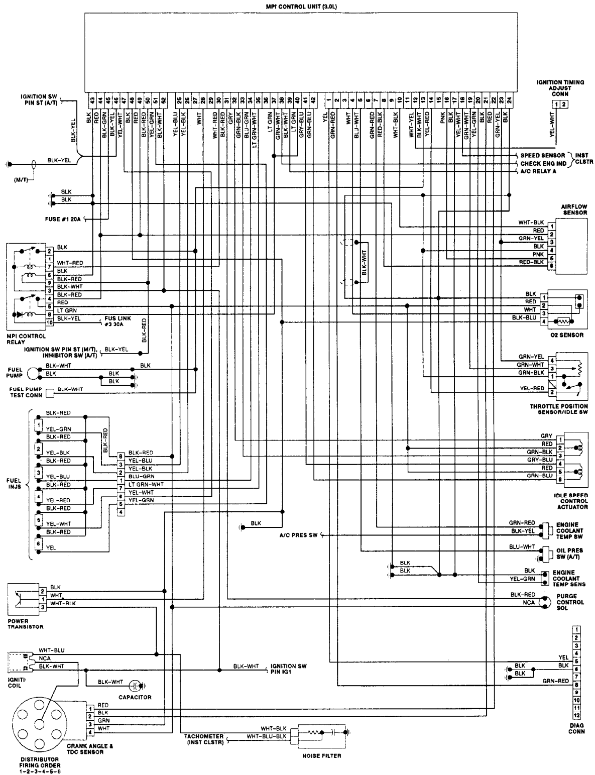
Fig. 10: Wiring Diagram (Montero 3.0L)
