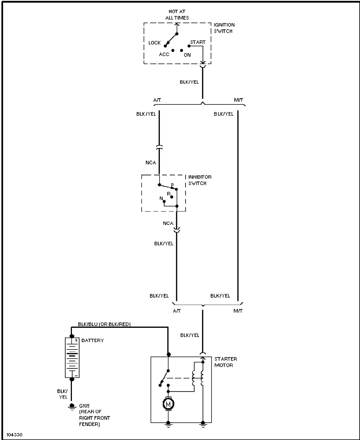
Starting Circuit
