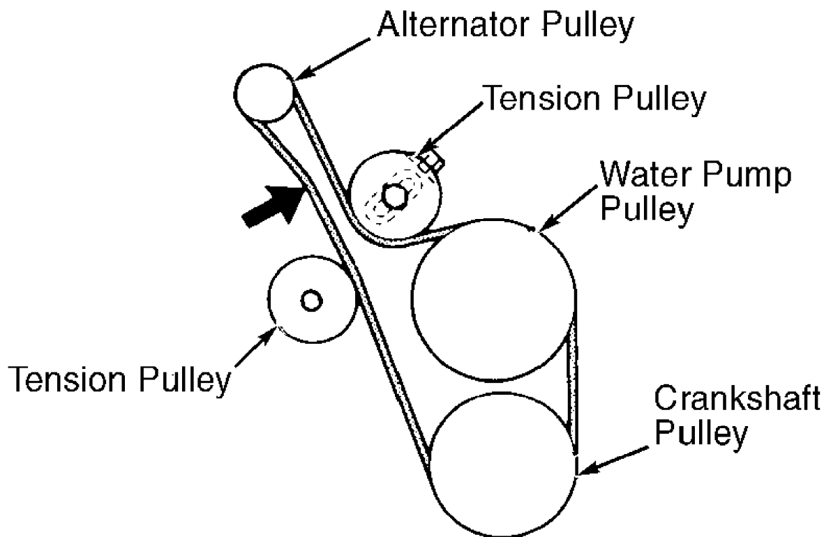
Fig. 1: Routing Serpentine Belt Courtesy of Mitsubishi Motor Sales of America.
