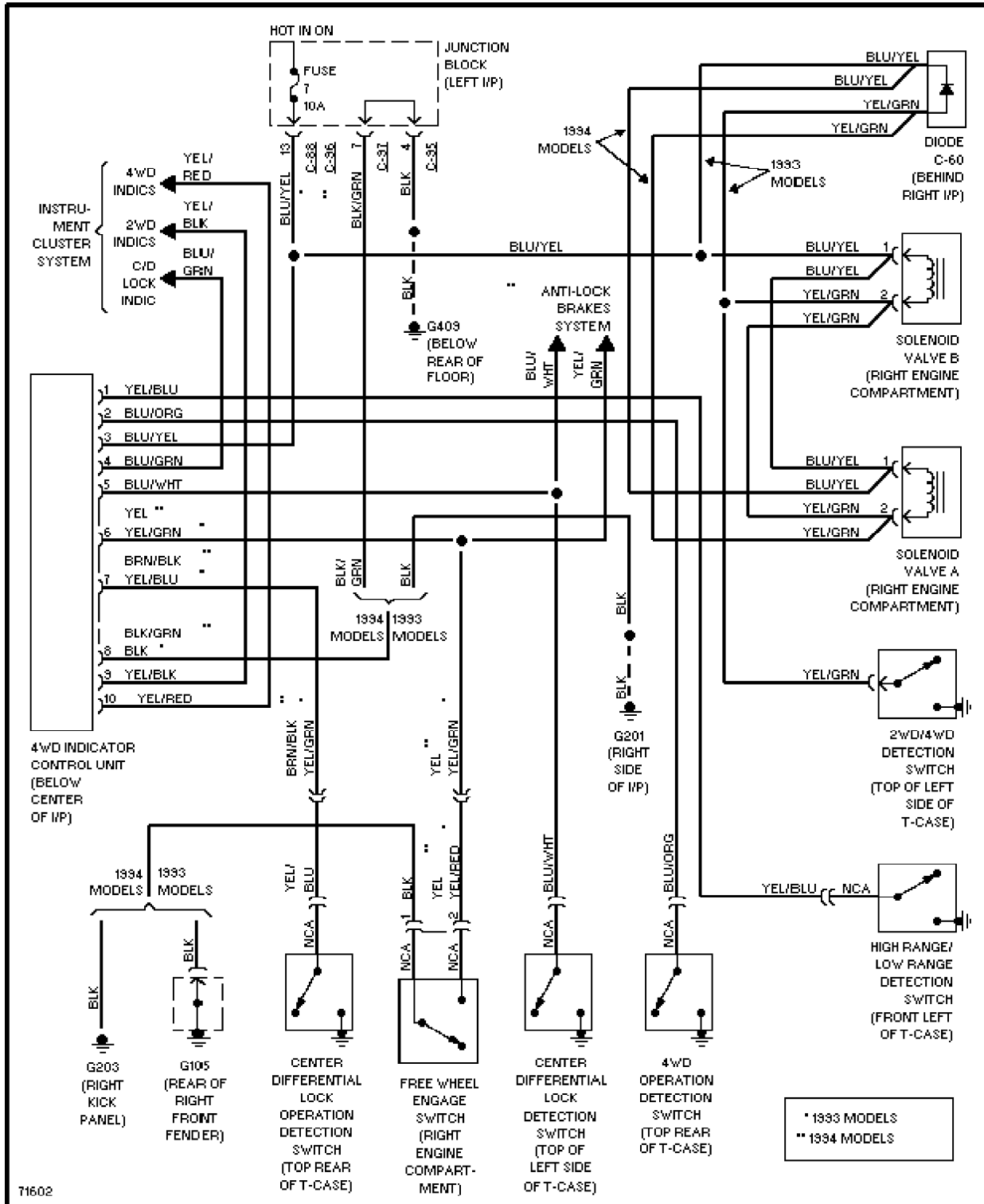
Active Trac 4WD Circuit
