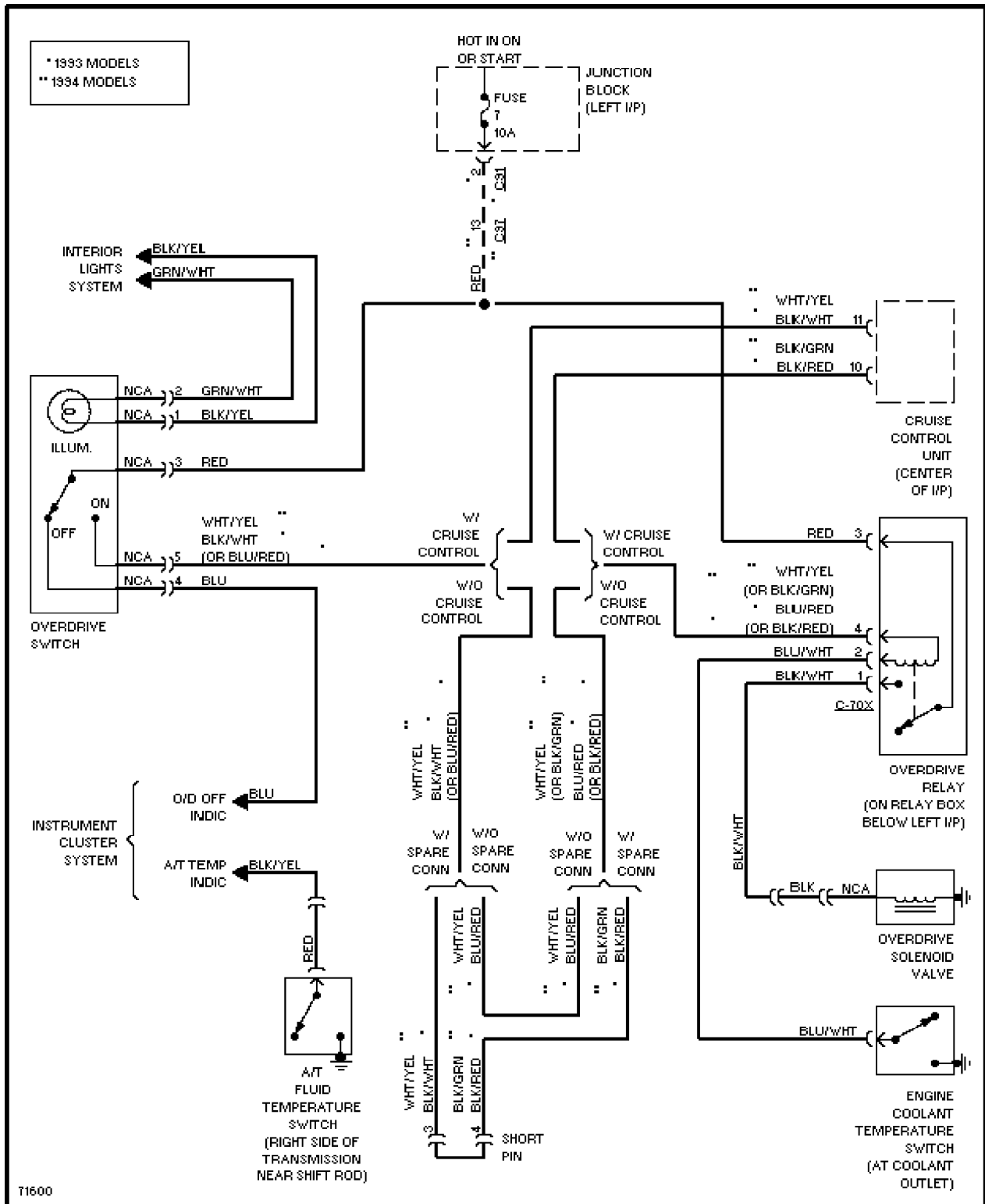
Transmission Circuit
