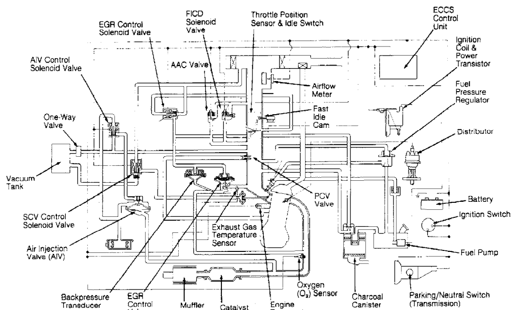
Fig. 3: Pickup (4-Cylinder) Vacuum Diagram Courtesy of Nissan Motor Co., U.S.A.
