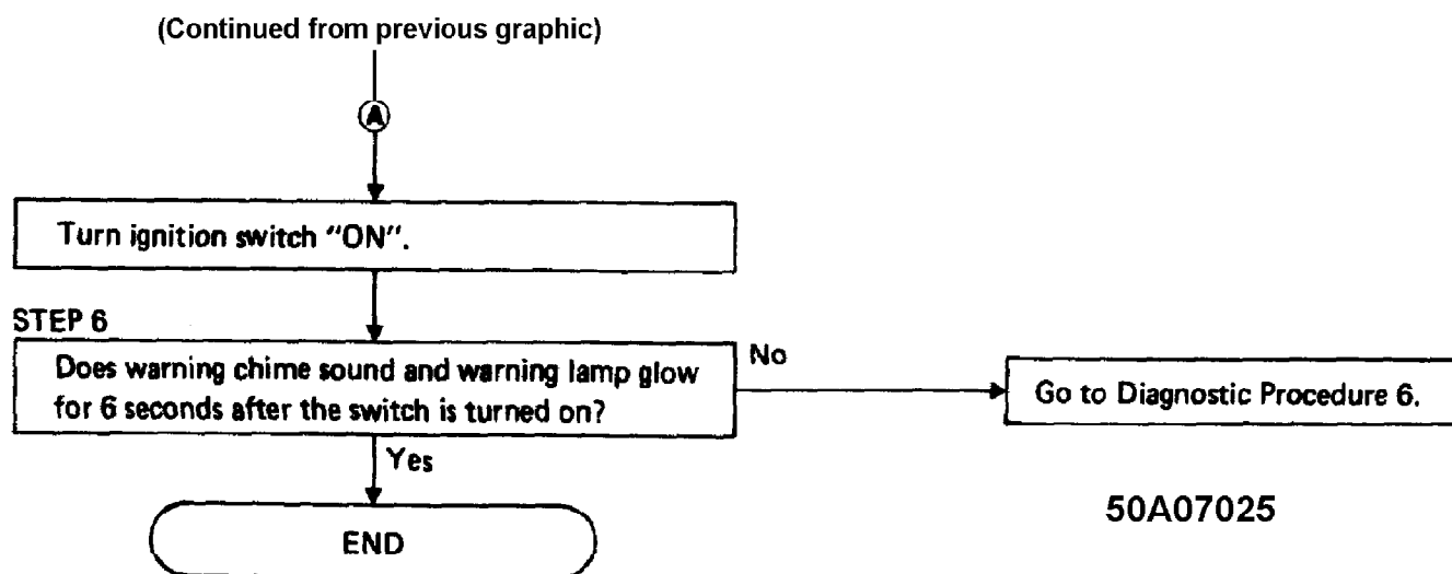
Fig. 17: Diagnostic Procedure 2 (Preliminary Check - 2 of 2)
