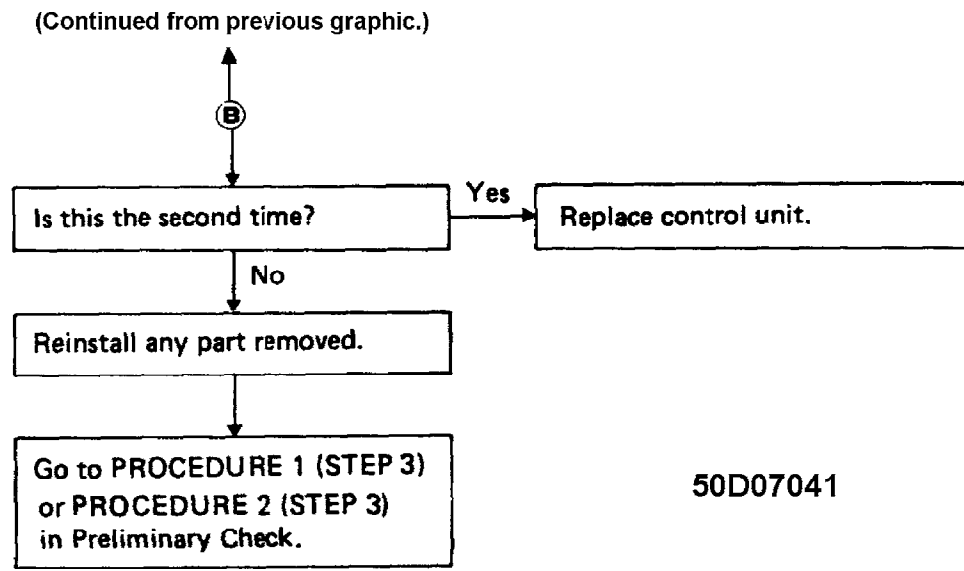
Fig. 26: Diagnostic Procedure 4 (2 of 2)
