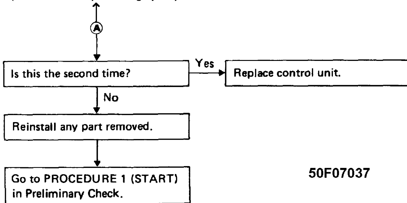
Fig. 22: Diagnostic Procedure 2 (2 of 2)
