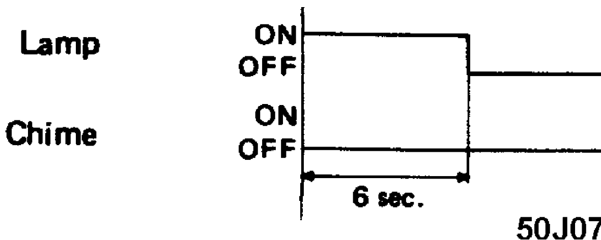
Fig. 13: NORMAL (All Belts Fastened & Shoulder Anchors In Rear Lock Position); Ignition Sw. OFF to ON
