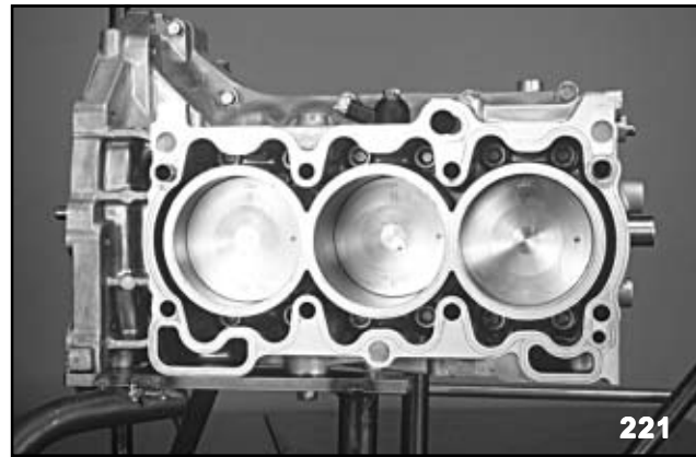
Engine Block Assembly Bolts (Right Bank)
