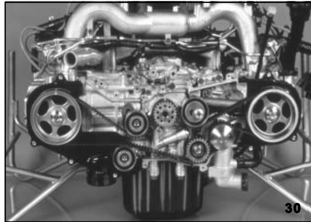
Mark Cam Belt
