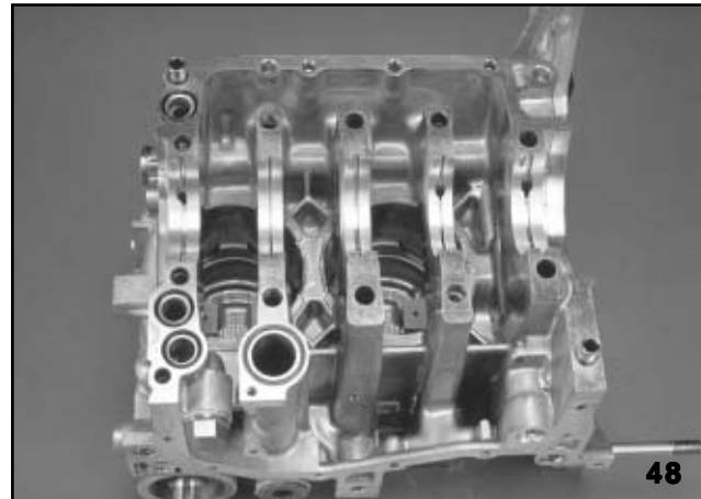
Crankcase Half with O-Rings
