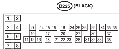
RELAY BLOCK
