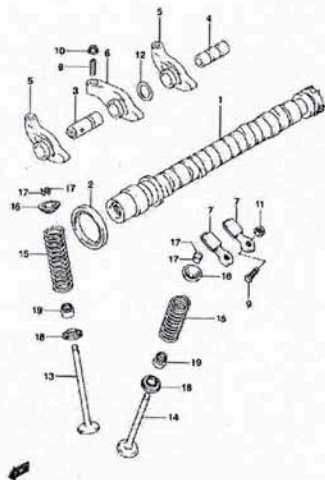
Camshaft-Valves (4V)
