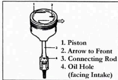
Piston Assembly
