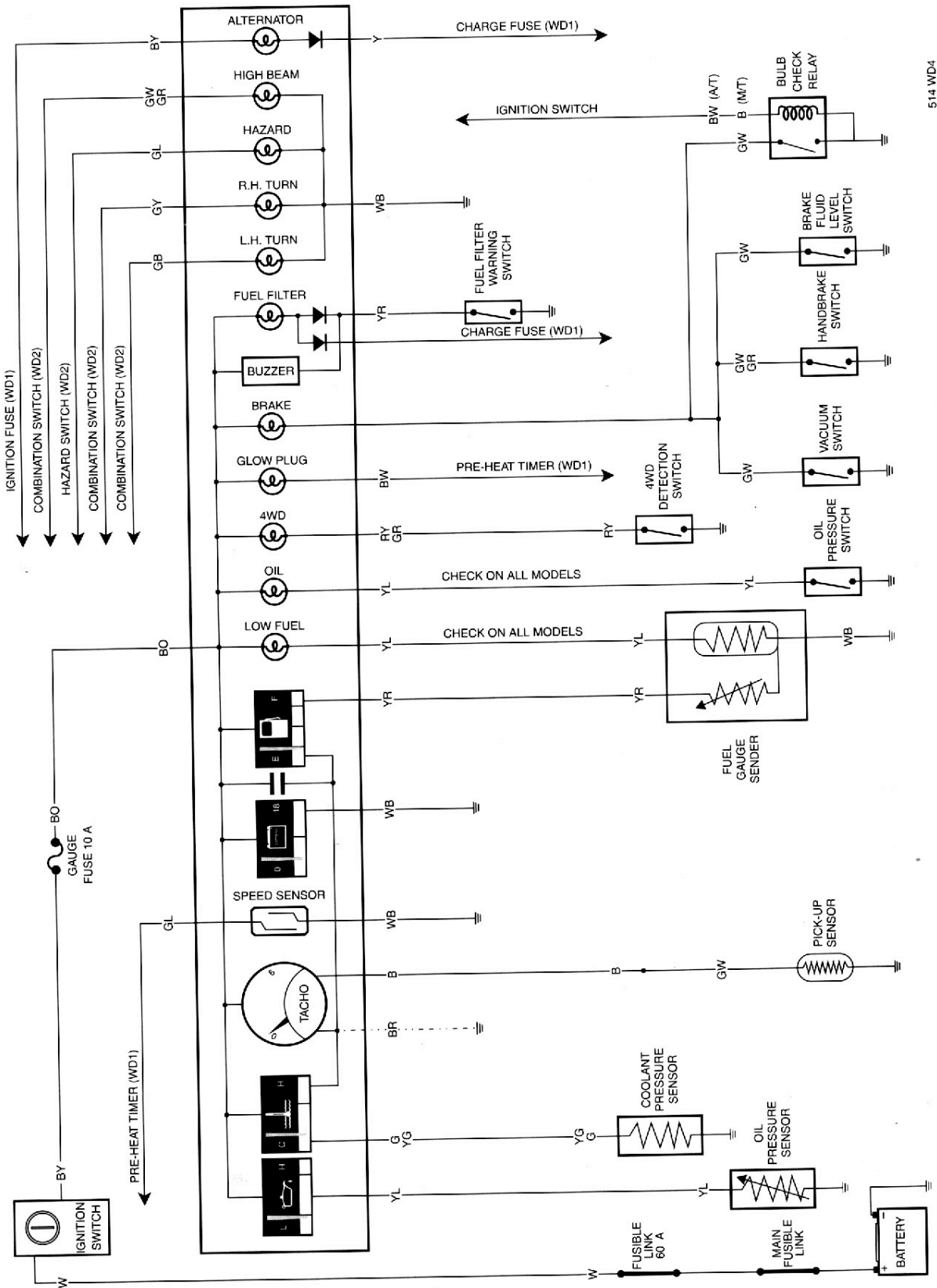
Instrument cluster.
