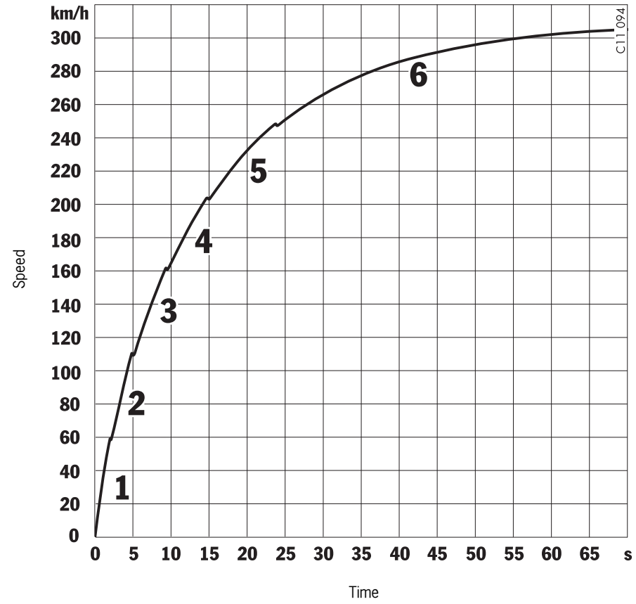
Acceleration diagram Manual transmission
