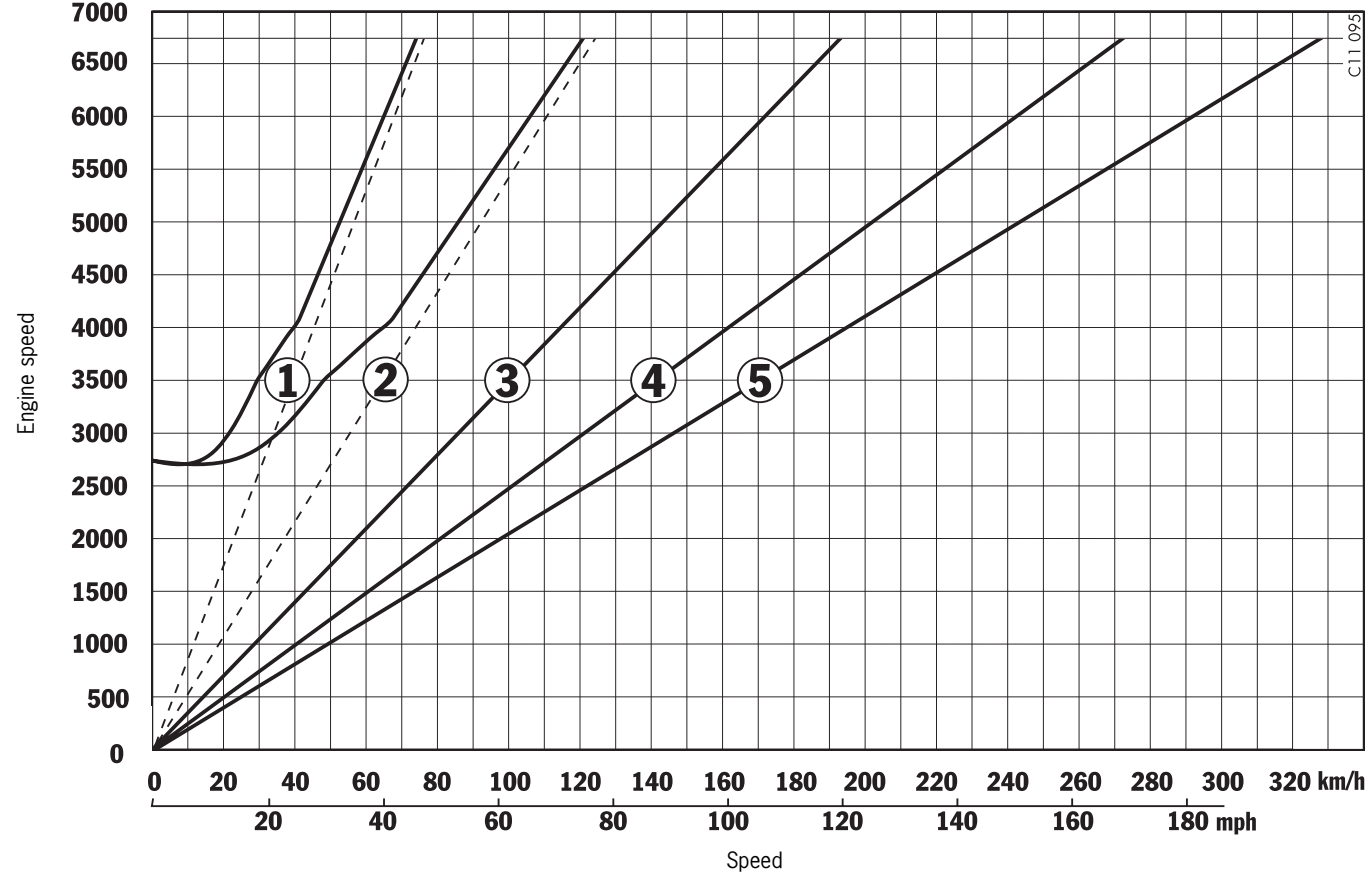
Transmission diagram Tiptronic
