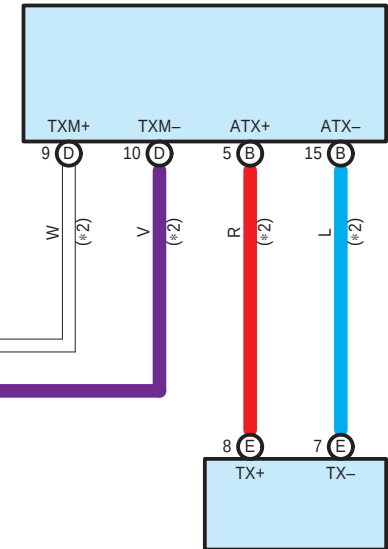
H55(E) Stereo Component Amplifier Assembly
