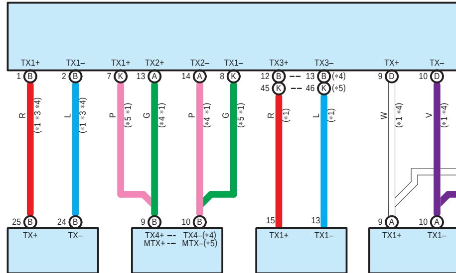
H9(B) Parking Assist ECU
