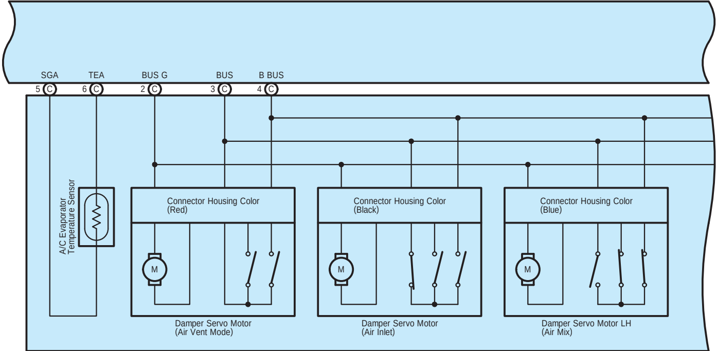
z1(C) A/C Blower Assembly
