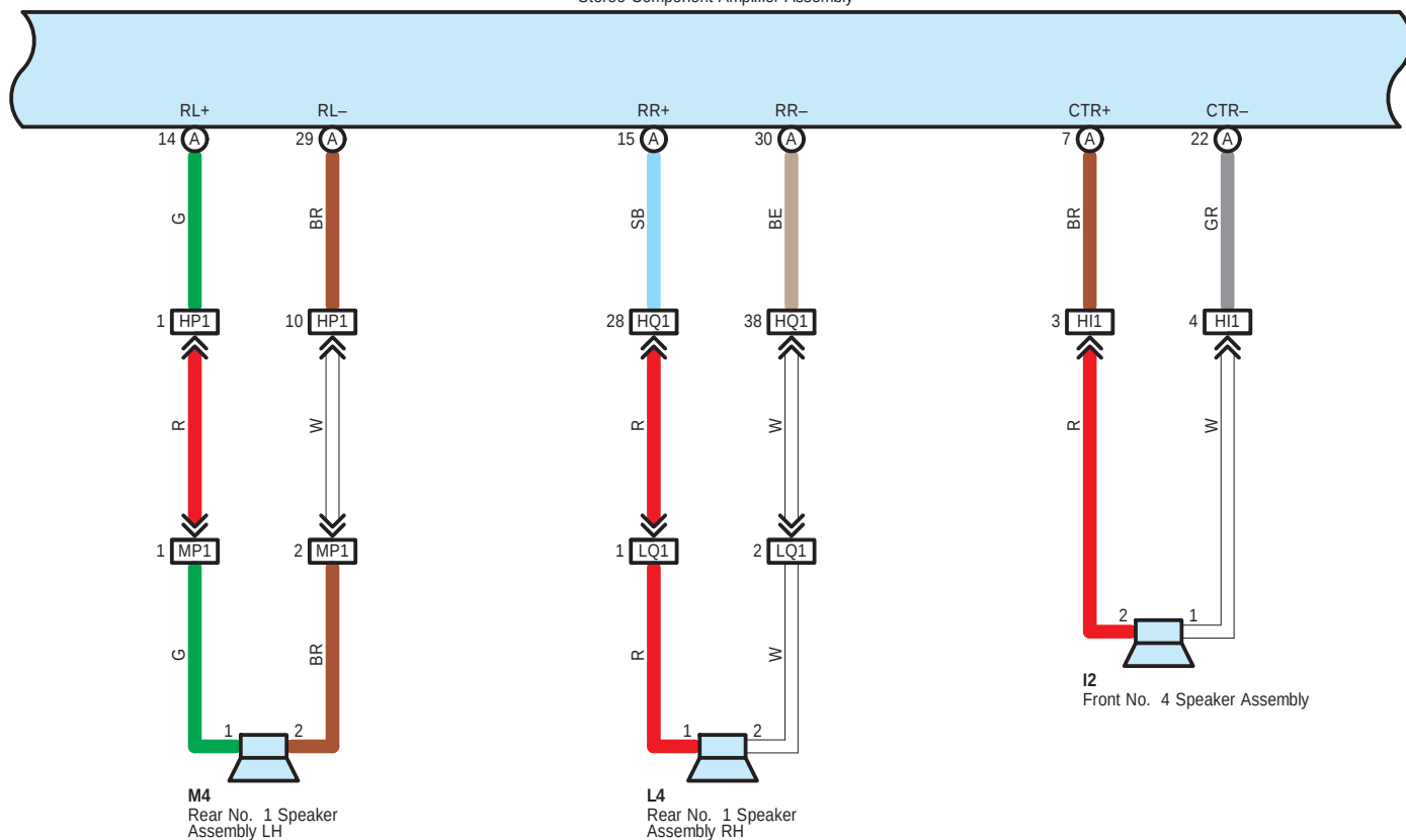
H157(A), H168(B) Stereo Component Amplifier Assembly
