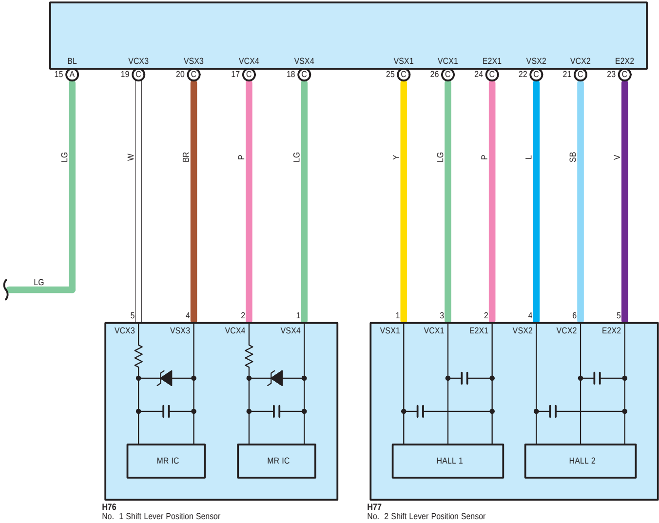
A19(A), H3(C) Power Management Control ECU
