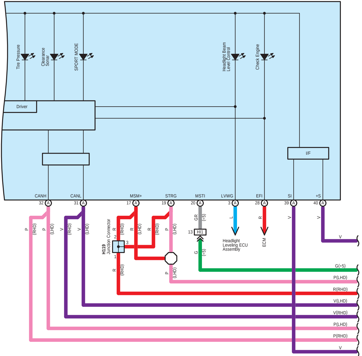
H19(A), H177(B) Combination Meter Assembly
