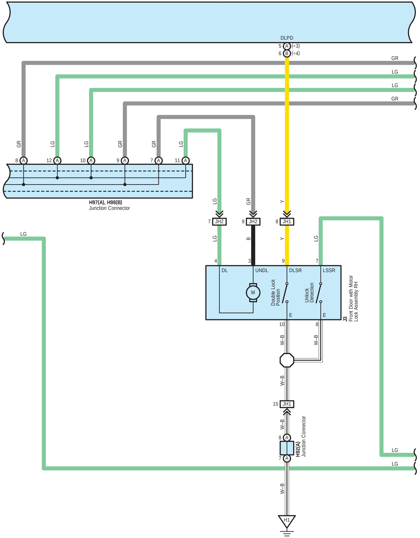
H140(A), H180(B) Double Lock Door Control Relay Assembly
