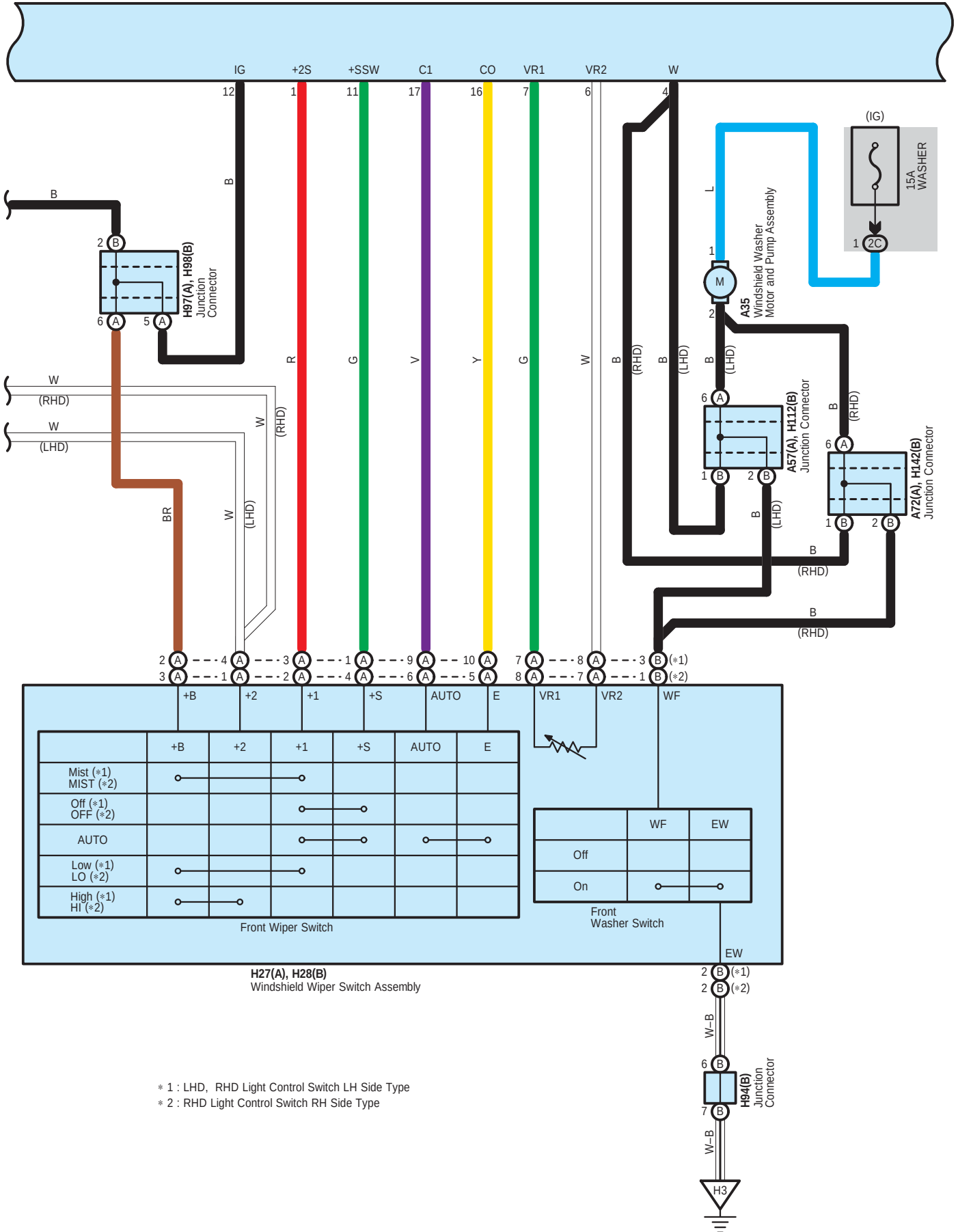
H75 Windshield Wiper Relay Assembly
