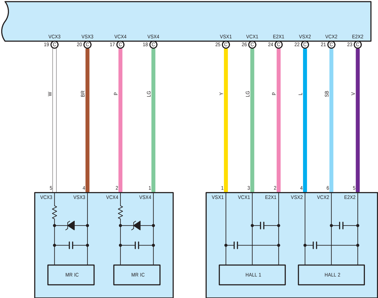
H76 No. 1 Shift Lever Position Sensor
