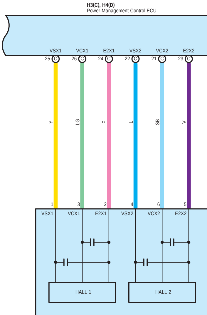
H77 No. 2 Shift Lever Position Sensor
