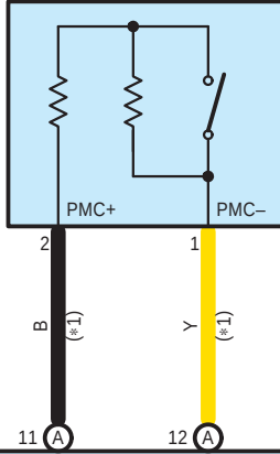
H134 Airbag Cut Off Switch Cylinder Sub-Assembly
