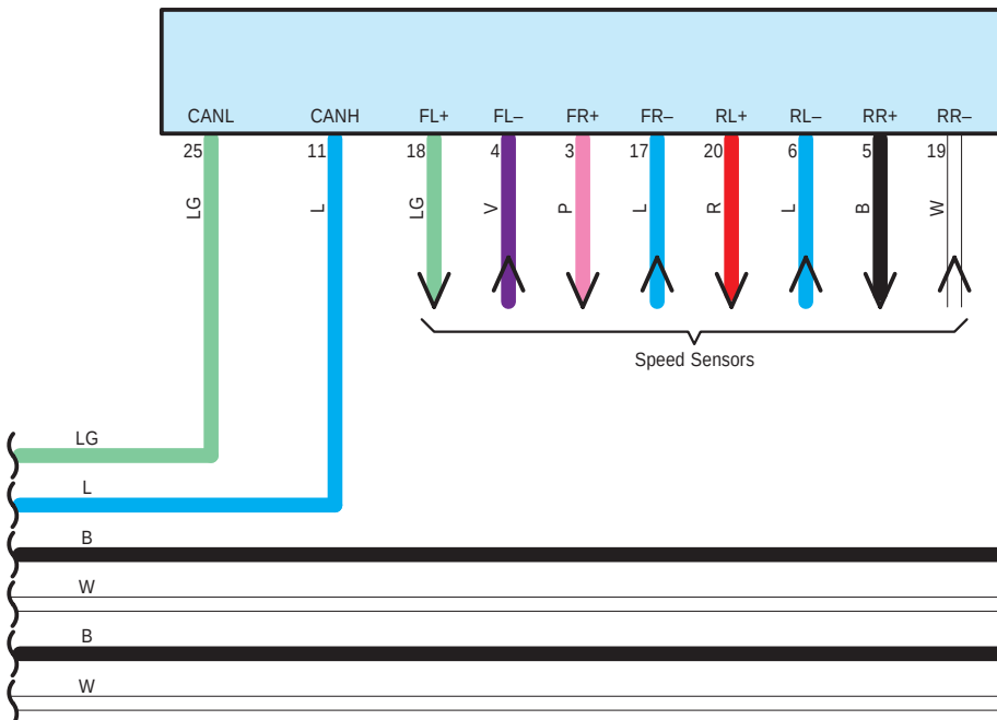
A36 Skid Control ECU with Actuator
