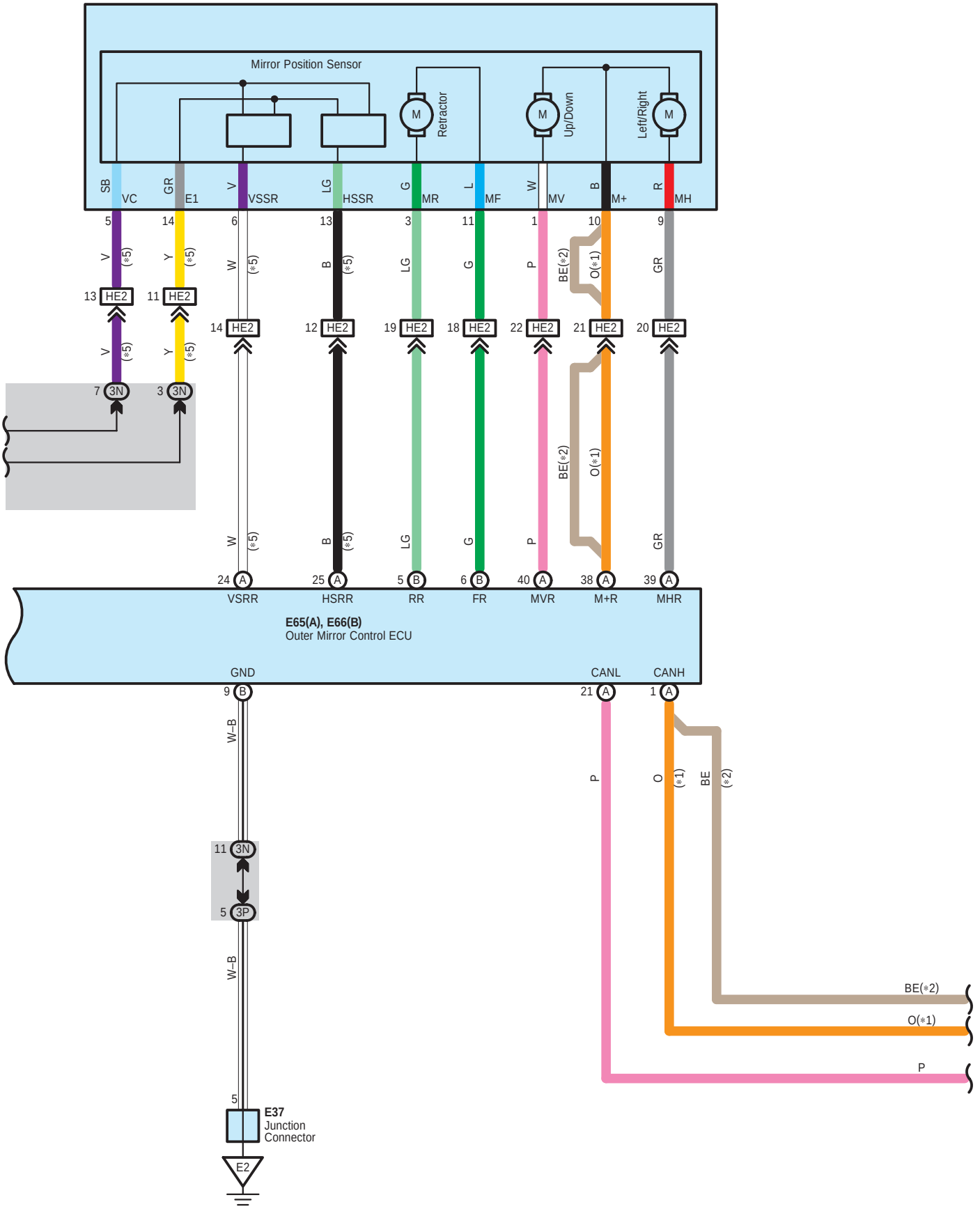
H4 Outer Rear View Mirror (RH)
