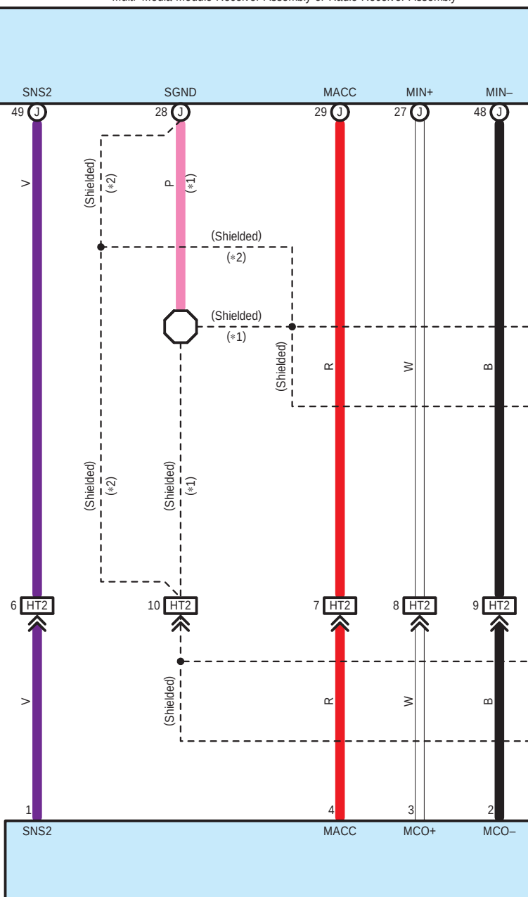
T11 Roof Console Box Assembly
