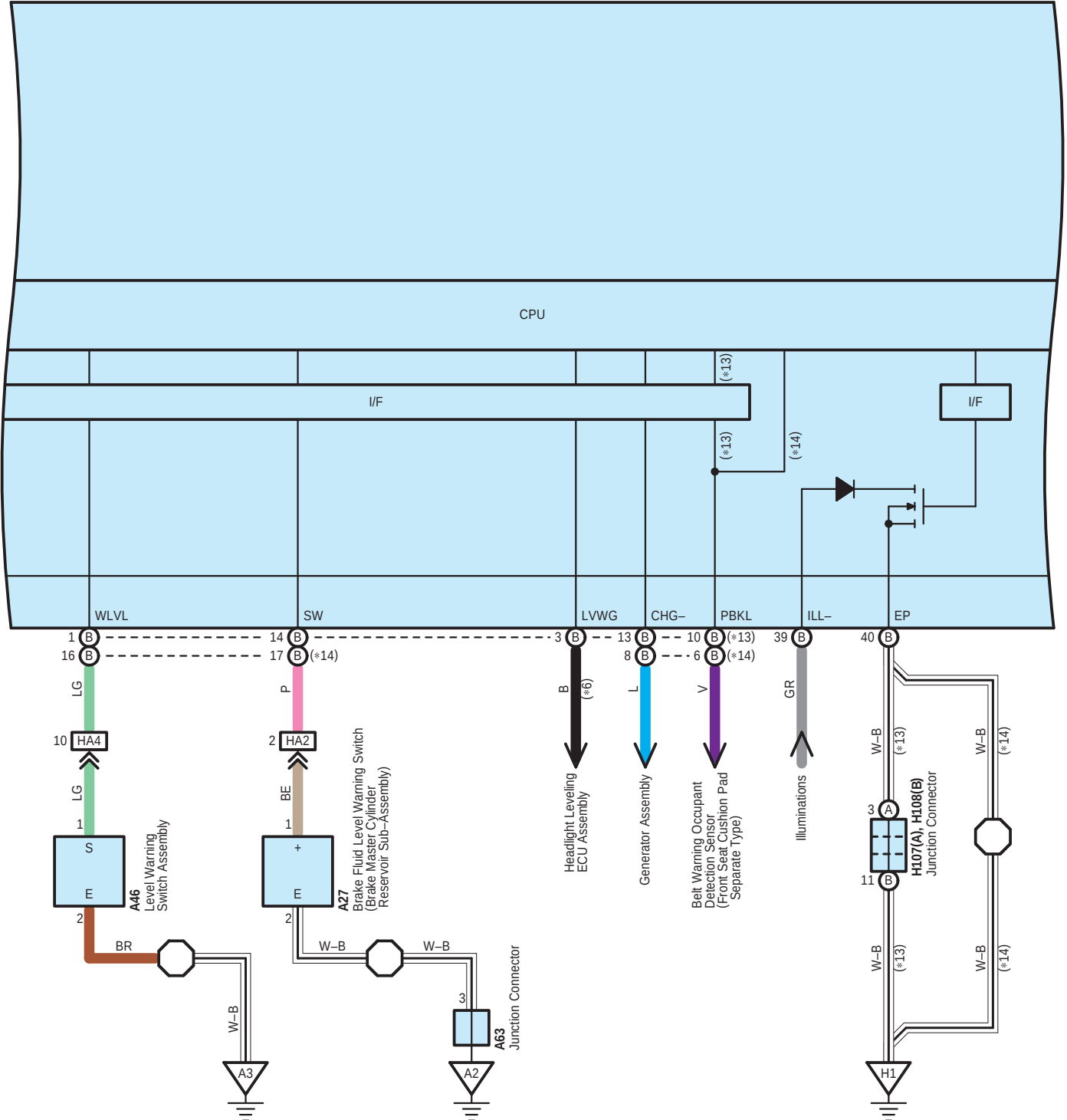
H13(A), H14(B), H210(C) Combination Meter Assembly
