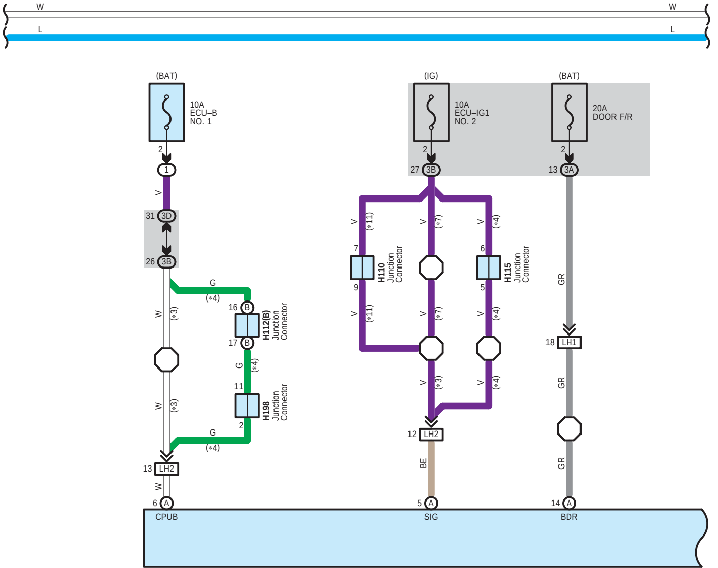
L10(A) Outer Mirror Control ECU Assembly RH
