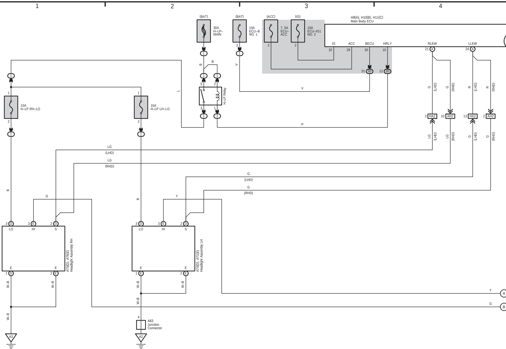
Headlight (From Jul. 2015 Production)
