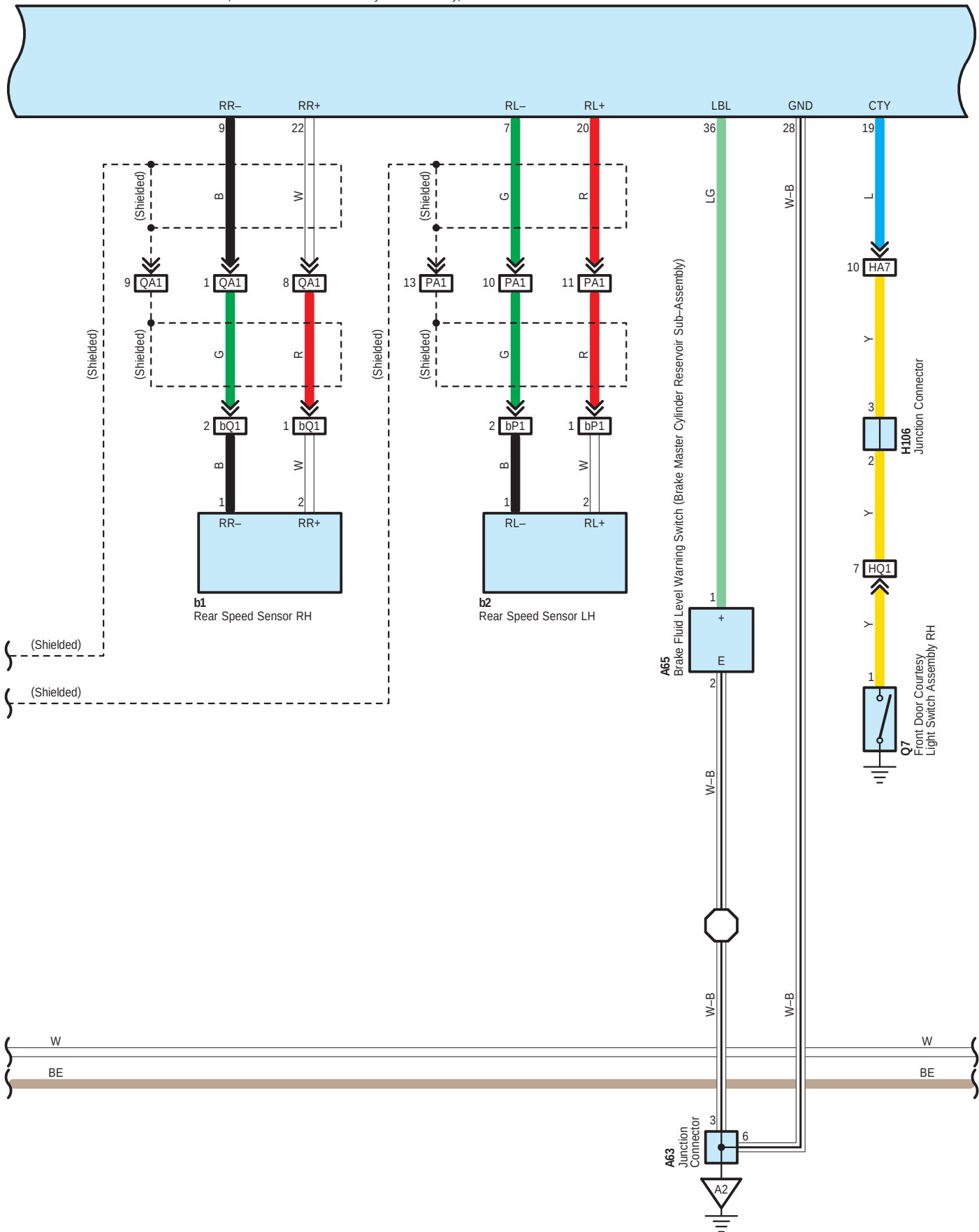
A24 Skid Control ECU with Actuator (Brake Booster with Master Cylinder Assembly)
