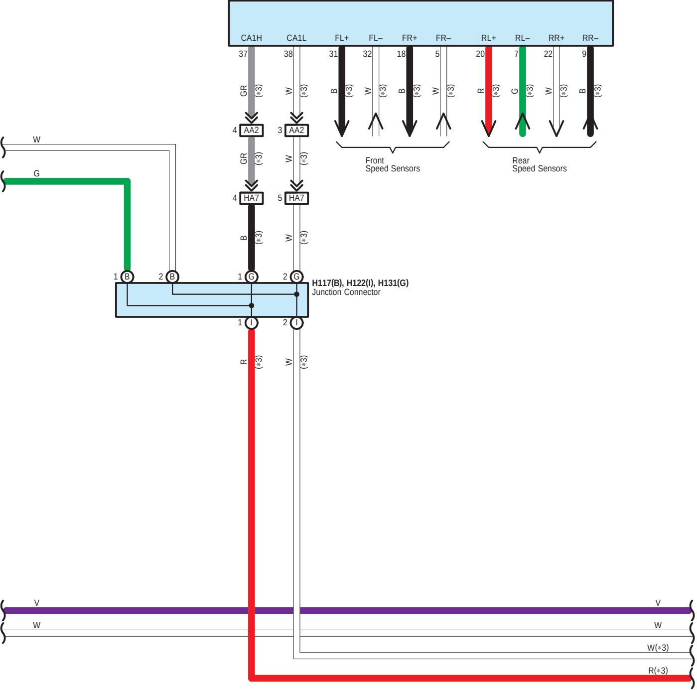
A24 Skid Control ECU with Actuator (Brake Booster with Master Cylinder Assembly)
