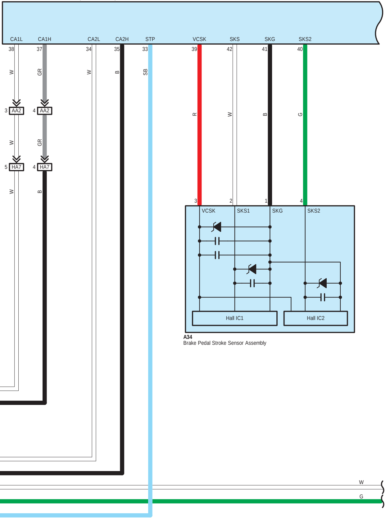
A24 Skid Control ECU with Actuator (Brake Booster with Master Cylinder Assembly)
