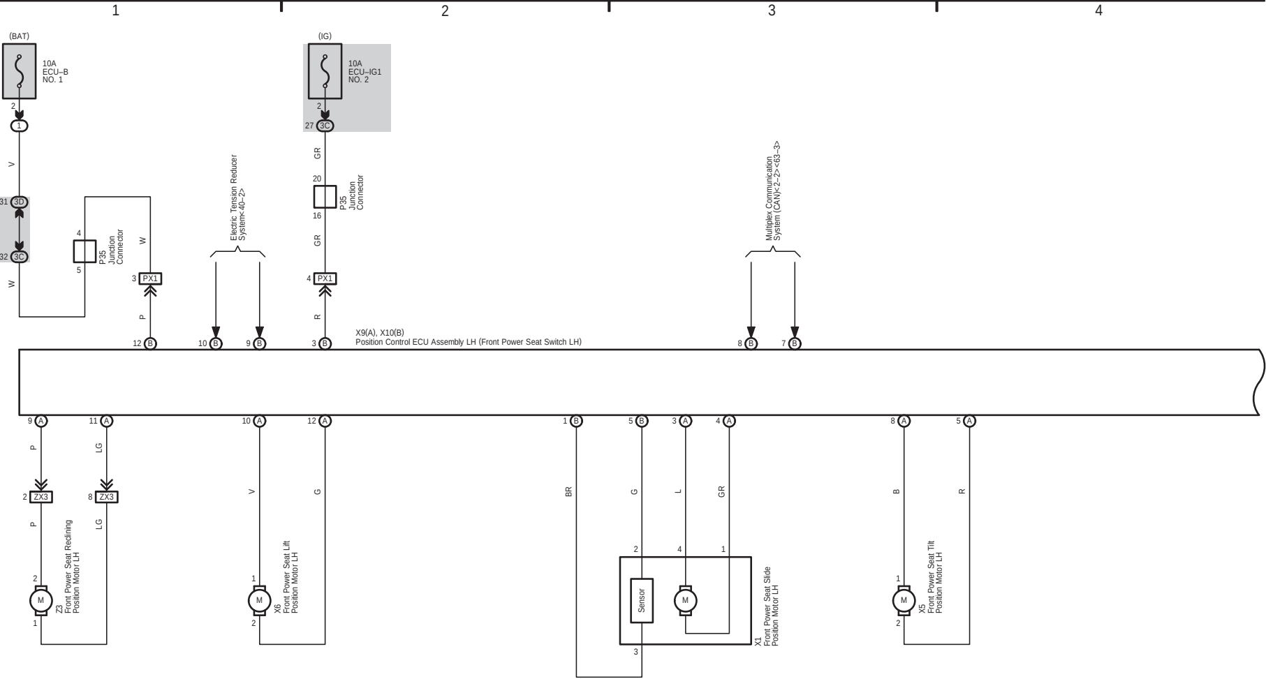
Power Seat (LHD Driver' s Seat w/ Seat Position Memory) (From Aug. 2014 Production)
