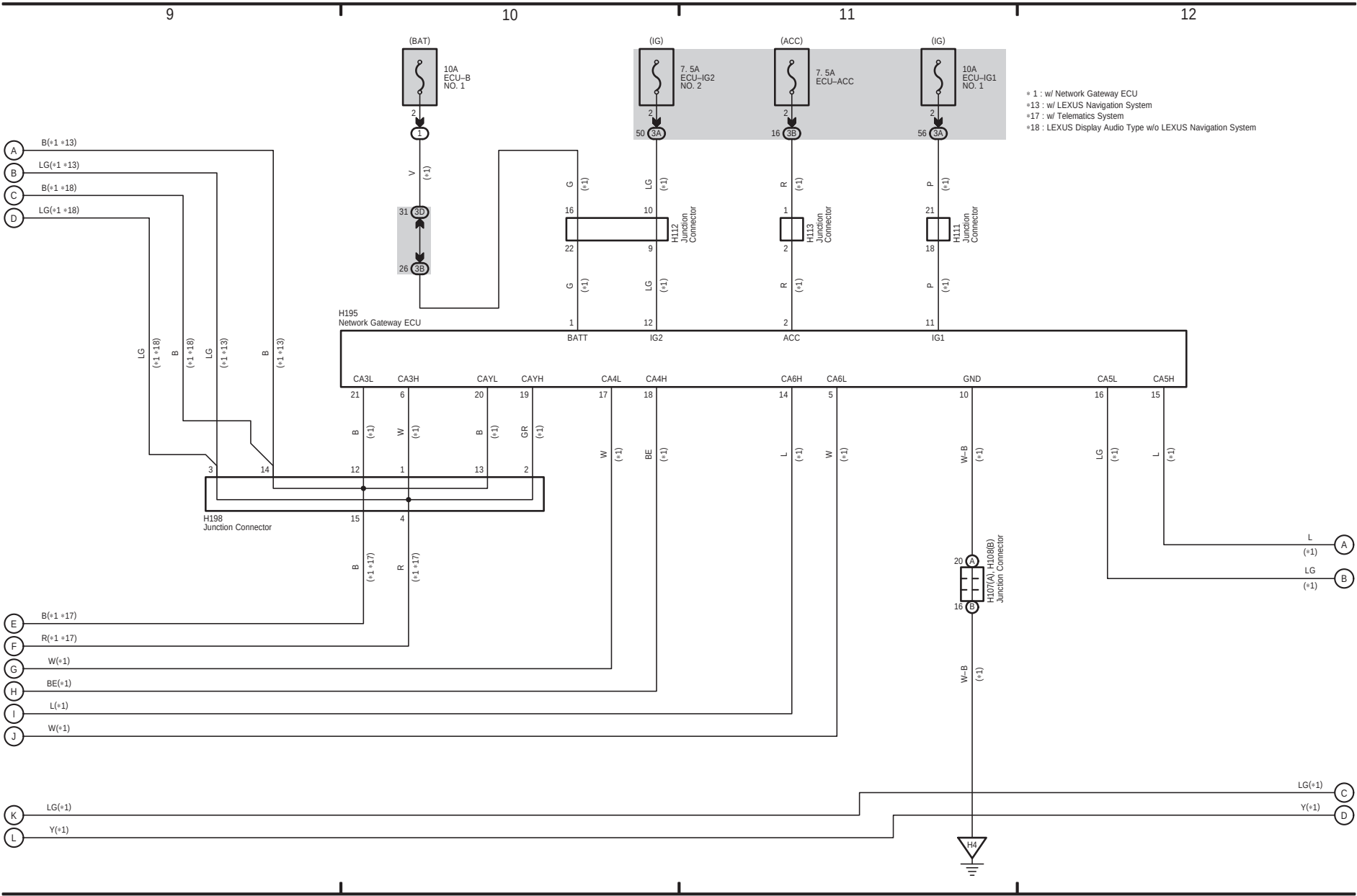
Multiplex Communication System (CAN) (LHD) (From Jul. 2015 Production)
