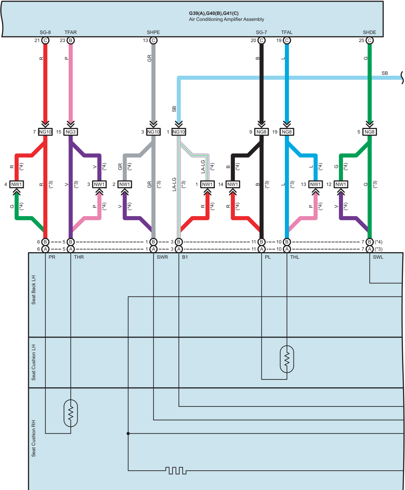
N111(A), W1(B) Seat Heater Assembly (for Rear Seat)
