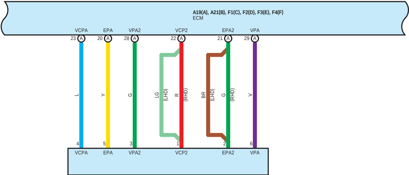
A2 Accelerator Pedal Sensor Assembly
