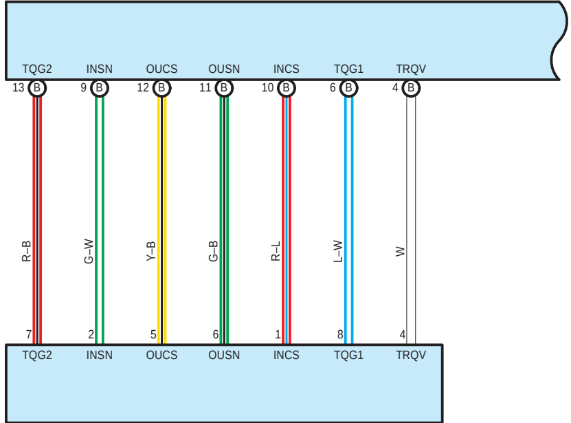
C3 Power Steering Torque Sensor (Power Steering Link Assembly)
