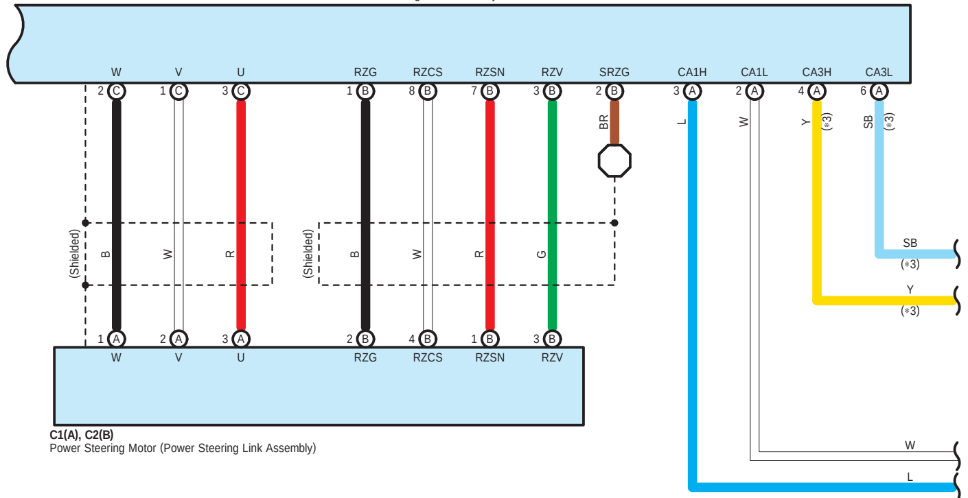
A29(A), C7(B), C8(C) Power Steering ECU Assembly
