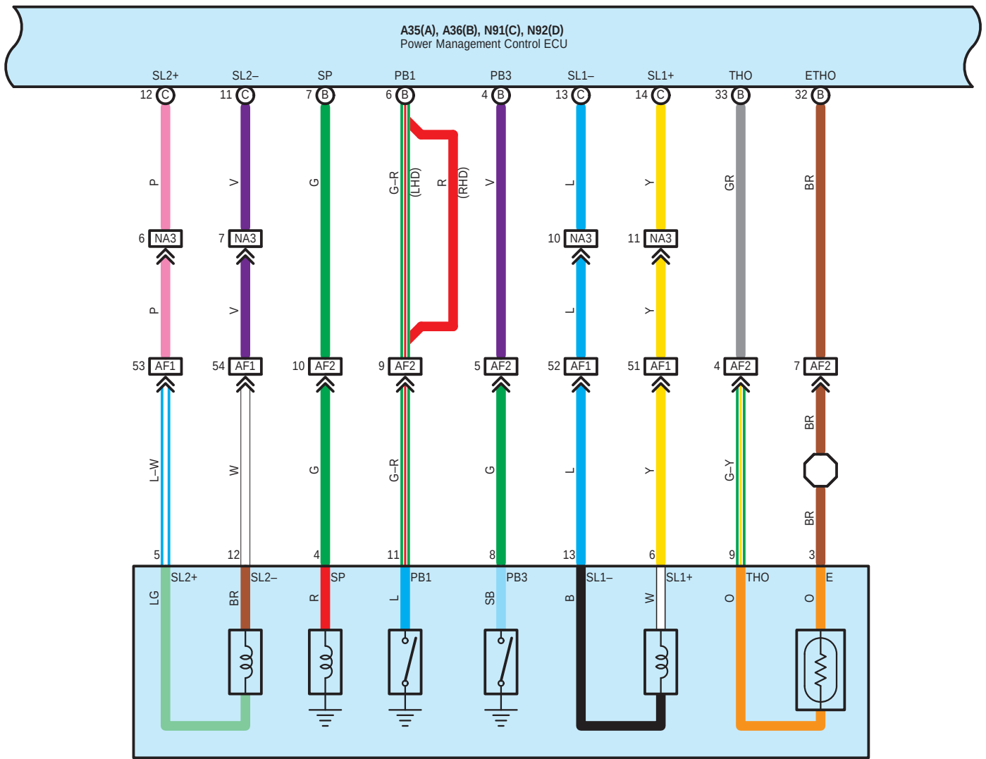
F52 Hybrid Vehicle Transmission (Transmission Wire)
