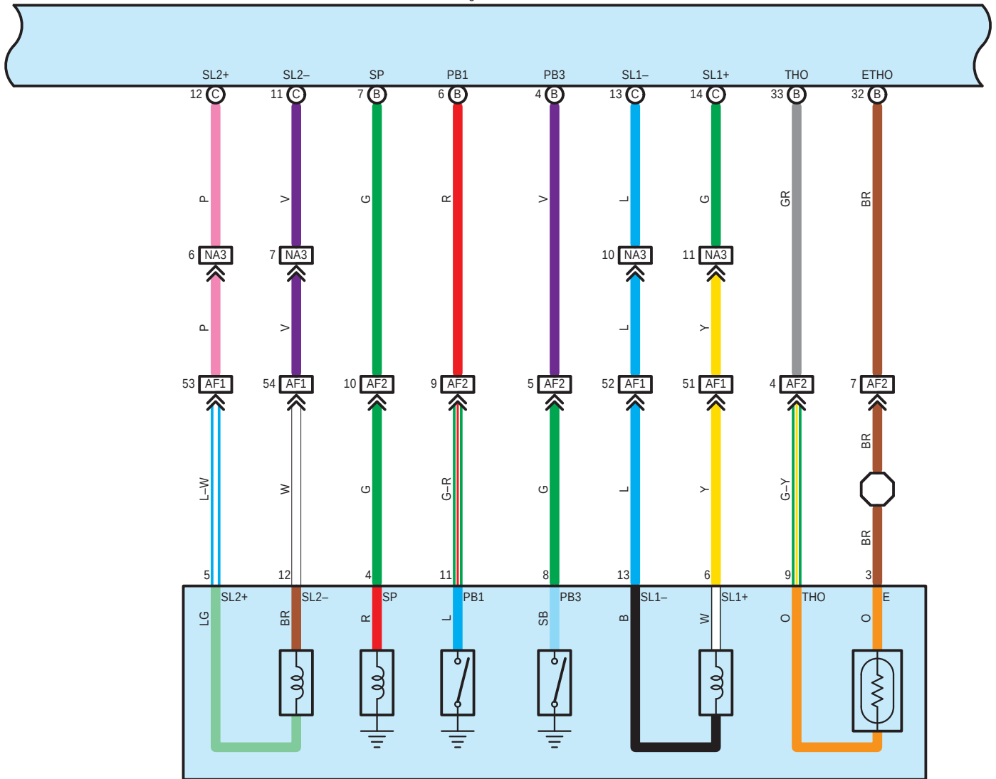
F52 Hybrid Vehicle Transmission (Transmission Wire)
