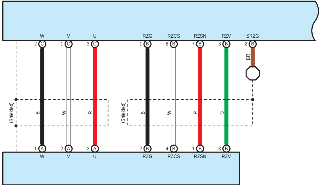
C1(A), C2(B) Power Steering Motor (Power Steering Link Assembly)
