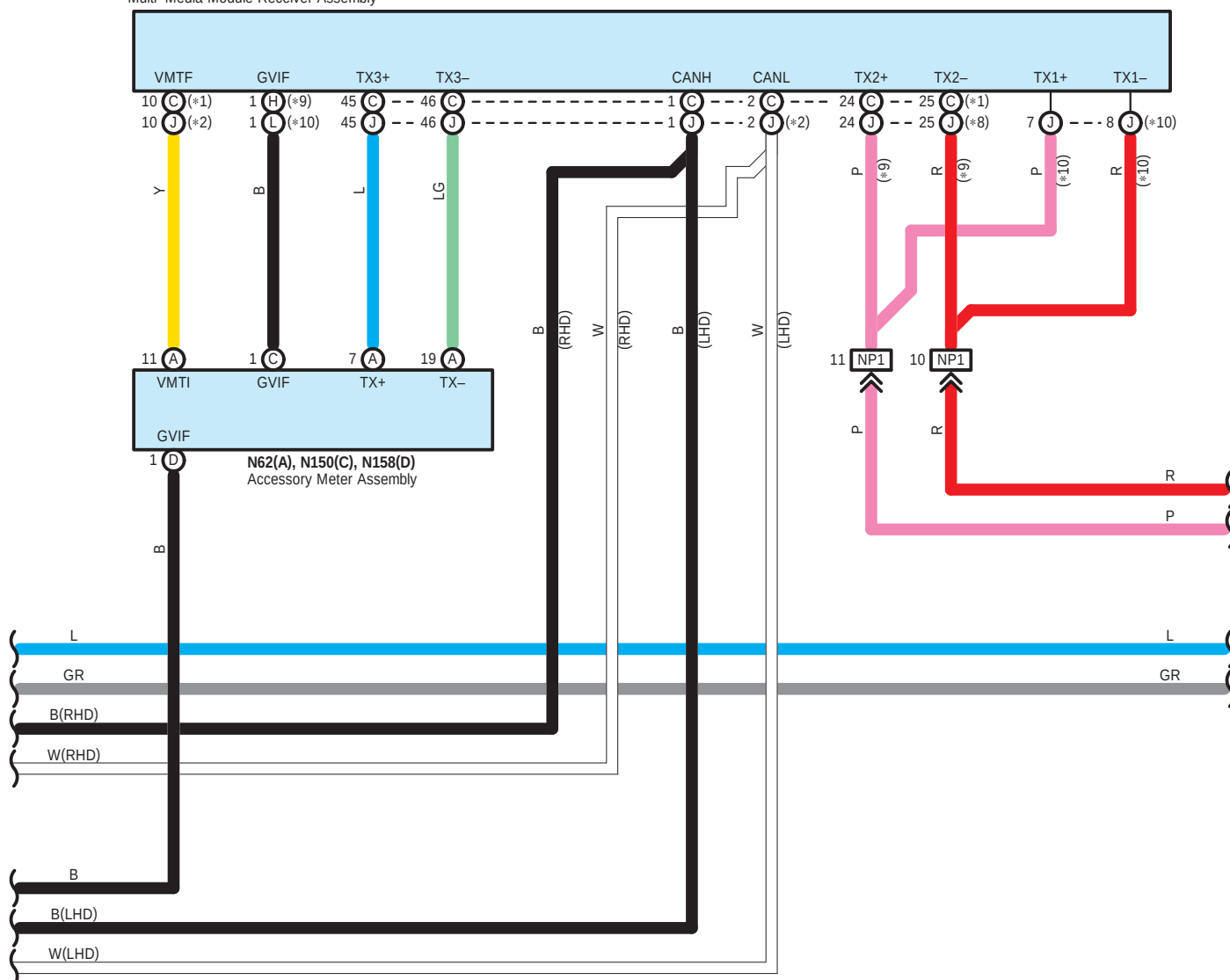
N68(C), N149(H), N164(J), N170(L) Multi-Media Module Receiver Assembly
