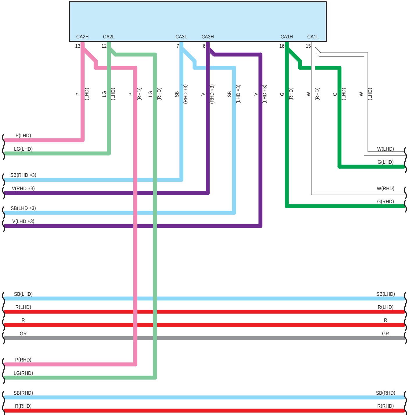
N82 Network Gateway ECU
