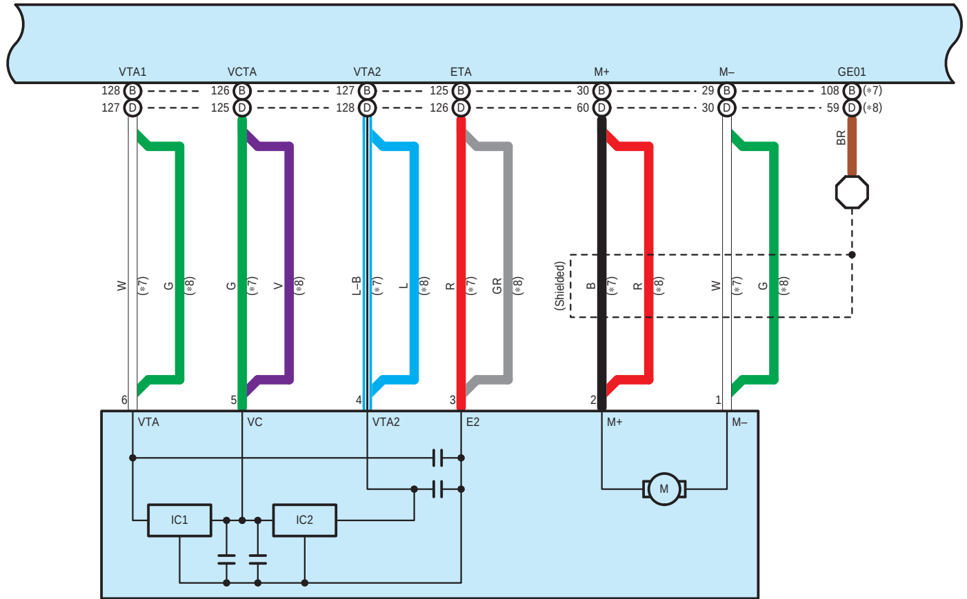
F24 Throttle Body with Motor Assembly
