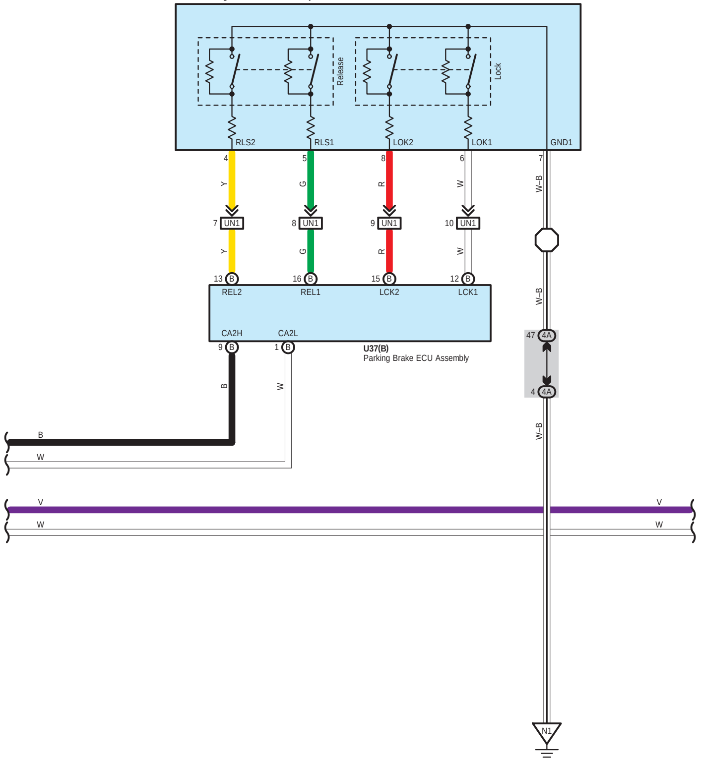
N23 Electric Parking Brake Switch Assembly
