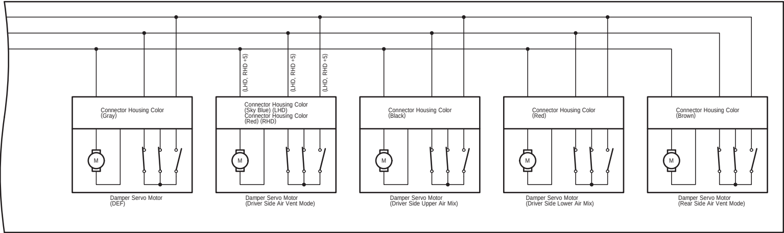
z1(C) Air Conditioner Harness Assembly
